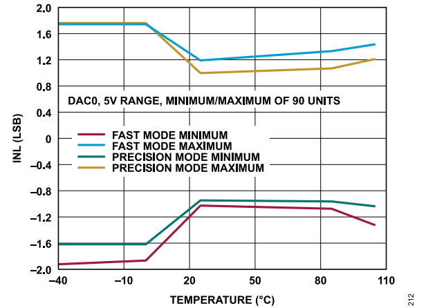
Figure 22. INL vs. Temperature
