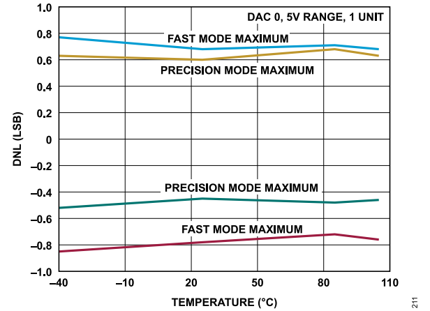
Figure 21. DNL vs. Temperature
