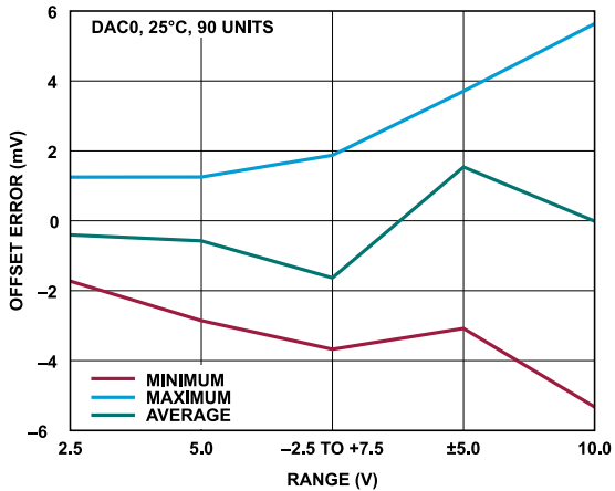
Figure 25. Offset Error vs. Range
