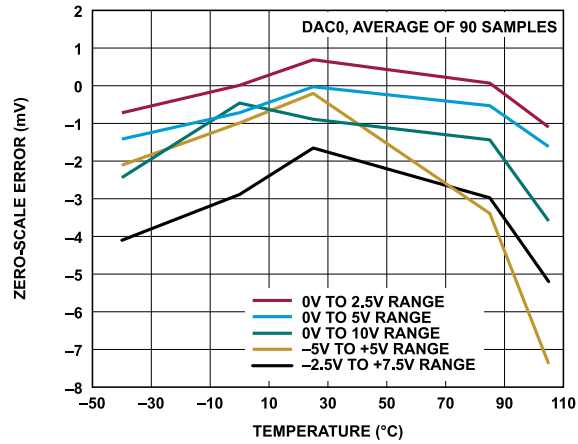
Figure 27. Zero-Scale Error vs. Temperature
