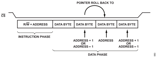
Figure 80. Looping Enabled with STREAM_MODE = 2
