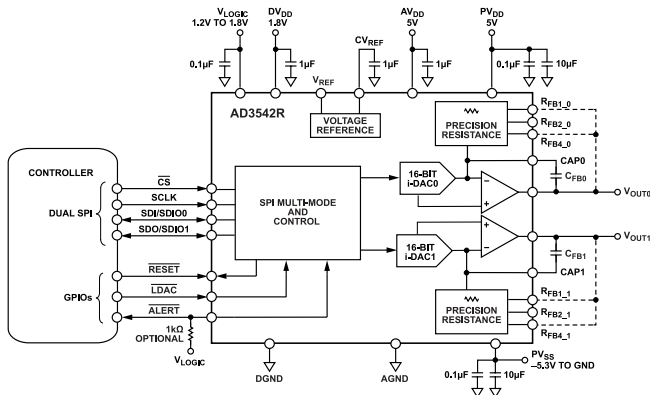
Figure 92. Recommended Application Circuit
