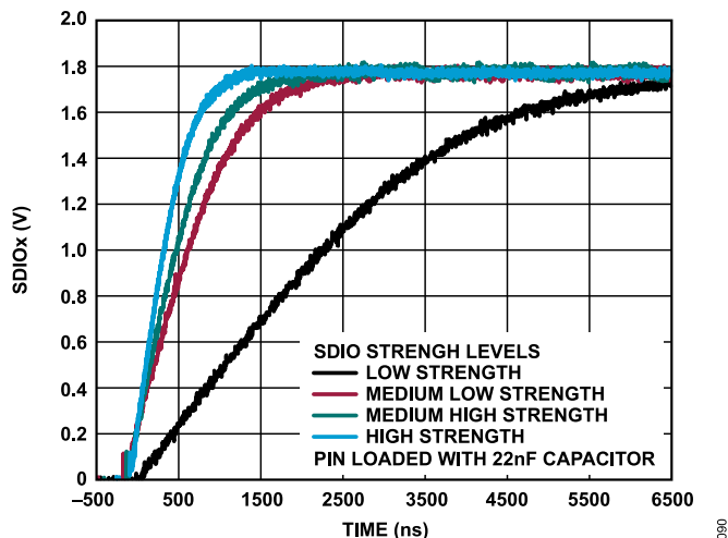
Figure 89. Driving Strength Options
