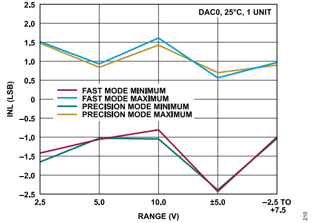
Figure 20. INL vs. Range, Fast Mode and Precision Mode
