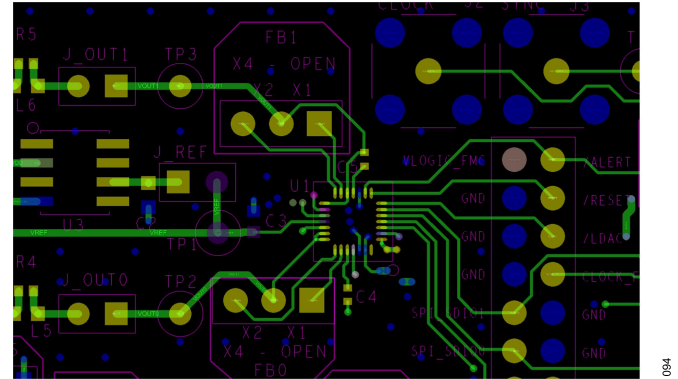
Figure 93. EVAL-AD3542R Component Arrangement and Layout
