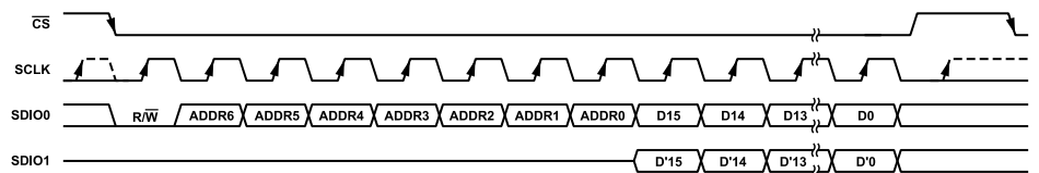
Figure 87. Synchronous Dual SPI Mode
