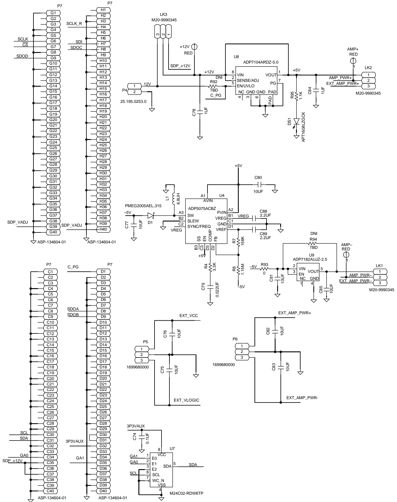
Figure 24. ADC Evaluation Board, Power Supply
