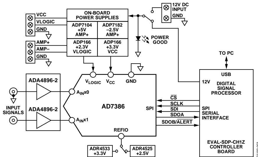
Figure 3. EVAL-AD7386FMCZ Functional Block Diagram
