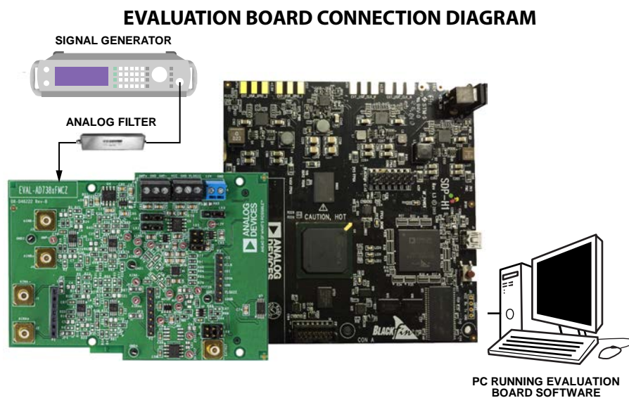
Figure 1. Typical Setup of the EVAL-AD7386FMCZ (Left) and the EVAL-SDP-CH1Z (Right)
