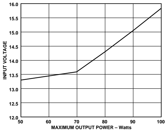
Figure 3. Low Line Dropout vs. Load at 90°C Case Temperature
