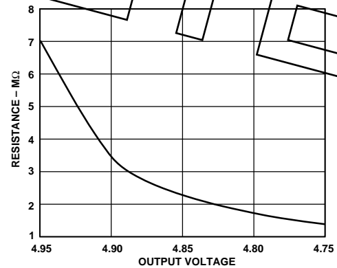
Figure 15. External Resistor Value for Reducing Output Voltage
