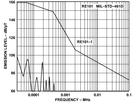
Figure 12. Radiated Emissions, MIL-STD-461D, RE101, 100 W Load
