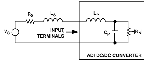
Figure 21. Model of Power Source and POL Converter Connection
