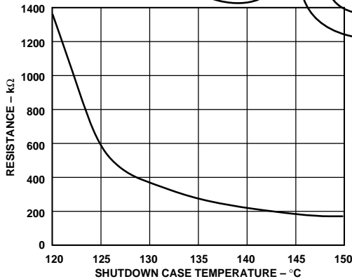
Figure 20. External Resistor Value for Raising Temperature Shutdown Point
