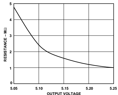
Figure 16. External Resistor for Increasing Output Voltage
