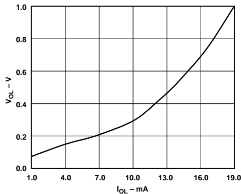
Figure 18. Sink Capability of Status Output
