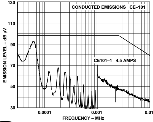
Figure 10. Conducted Emissions, MIL-STD-461D, CE101, +28 V Hot Line 100 W Load
