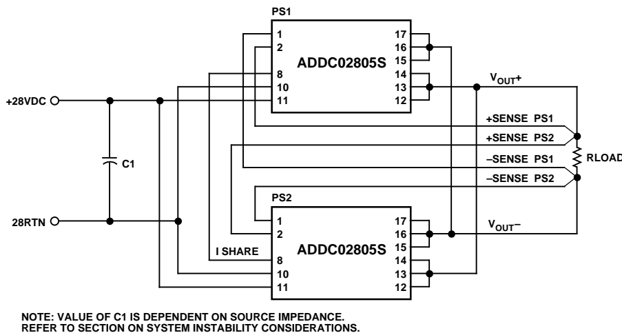
Figure 25. Typical Connections for Paralleling Two Converters
