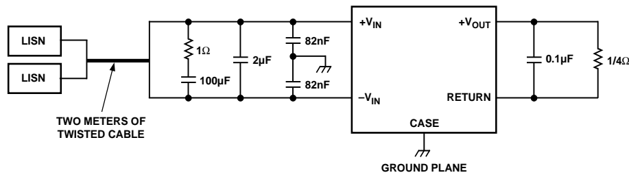
Figure 14. Schematic of Test Setup for EMI Measurements
