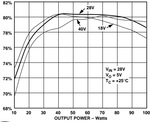
Figure 1. Efficiency vs. Line and Load at +25°C
