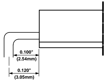
Figure 23. Minimum Bend Radius of 40 Mil (1.02 mm) Pins
