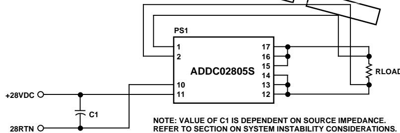
Figure 24. Typical Power Connections and External Parts for Converter
