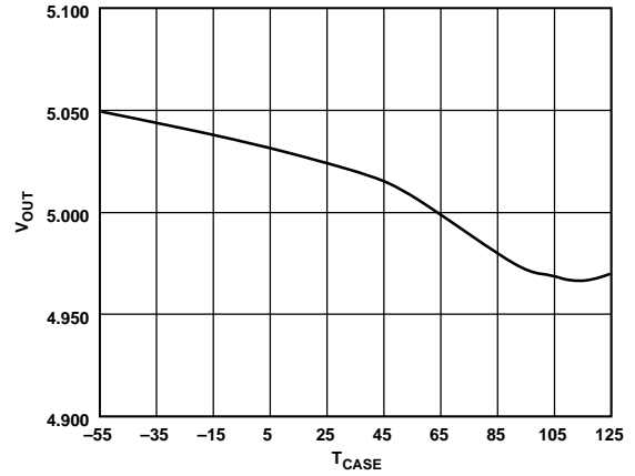
Figure 4. Output Voltage vs. Case Temperature (°C)
