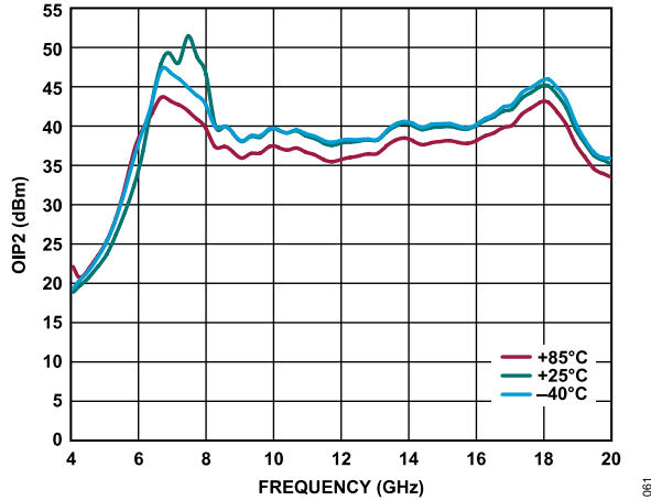
Figure 61. OIP2 vs. Frequency for Various Temperature, 4 GHz to 20 GHz, VDD = 3 V, IDQ = 90 mA, RBIAS = 909 Ω
