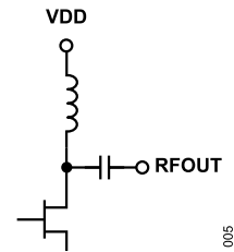
Figure 5. VDD and RFOUT Interface Schematic
