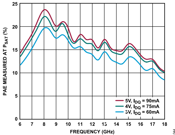
Figure 44. PAE Measured at P_{SAT} vs. Frequency for Various Supply Voltages and I_{DQ} , R_{BIAS} = 4.12\text{ k}\Omega
