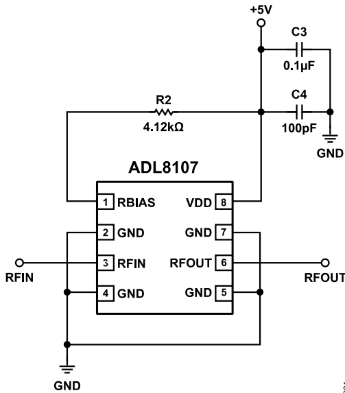
Figure 81. Typical Application Circuit
