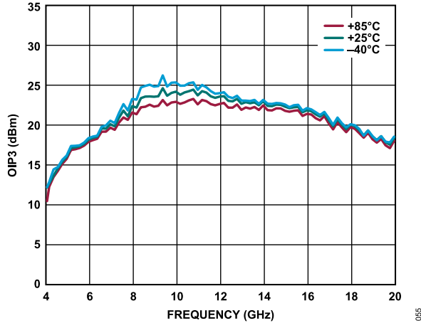
Figure 55. OIP3 vs. Frequency for Various Temperature, 4 GHz to 20 GHz, VDD = 3 V, IDQ = 90 mA, RBIAS = 909 Ω
