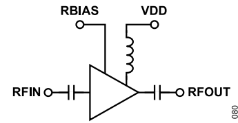
Figure 80. Simplified Schematic
