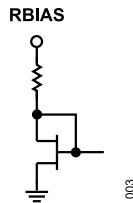
Figure 3. RBIAS Interface Schematic
