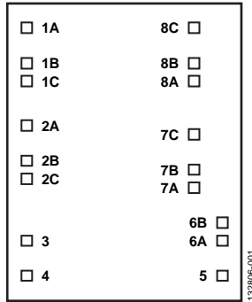
Figure 1. Pad Configuration
