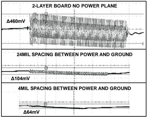
Figure 12. V_{DD} Voltage Noise for Various Stack-Up Options
