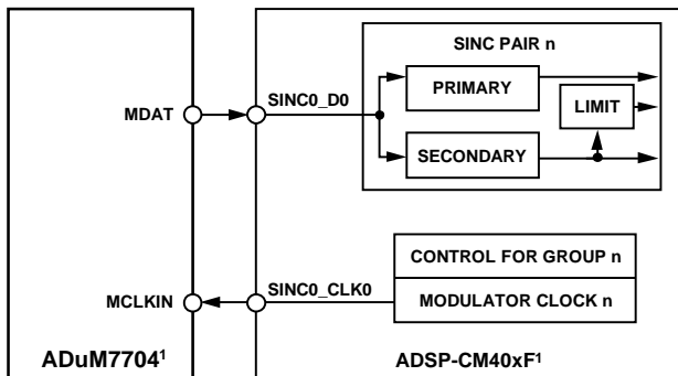
Figure 32. Interfacing the ADuM7704 to the ADSP-CM4xx
