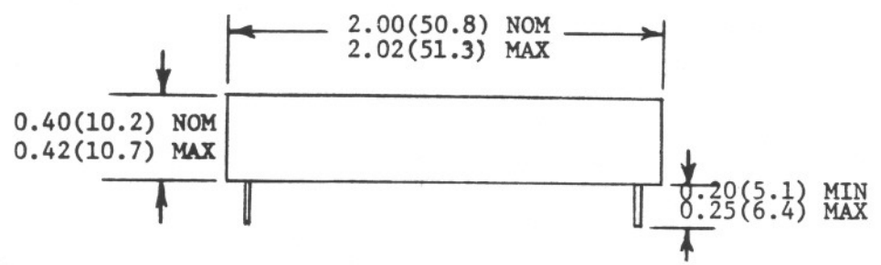
FIGURE 3 PHYSICAL OUTLINE
