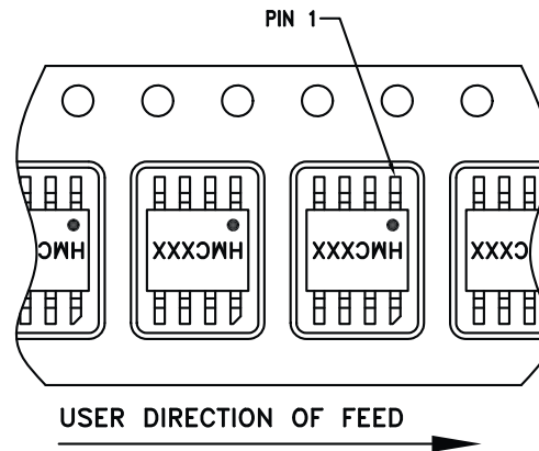
COMPONENT ORIENTATION (FORWARD TAPE AND REEL)
