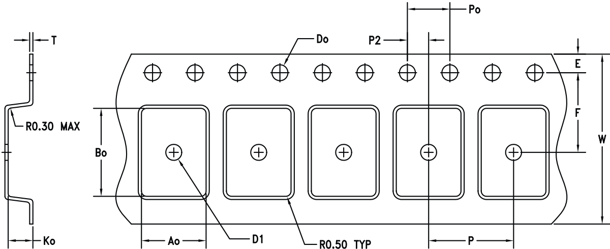
COMPONENT ORIENTATION (FORWARD TAPE AND REEL)
