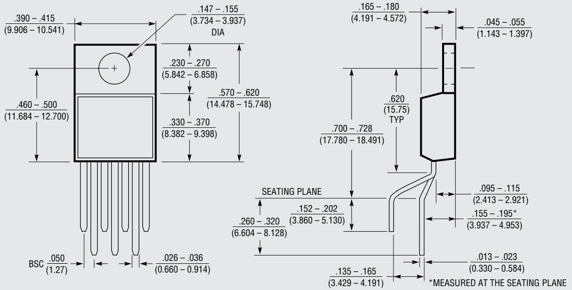
T7 Package 7-Lead Plastic TO-220 (Standard) (Reference LTC DWG # 05-08-1422)
