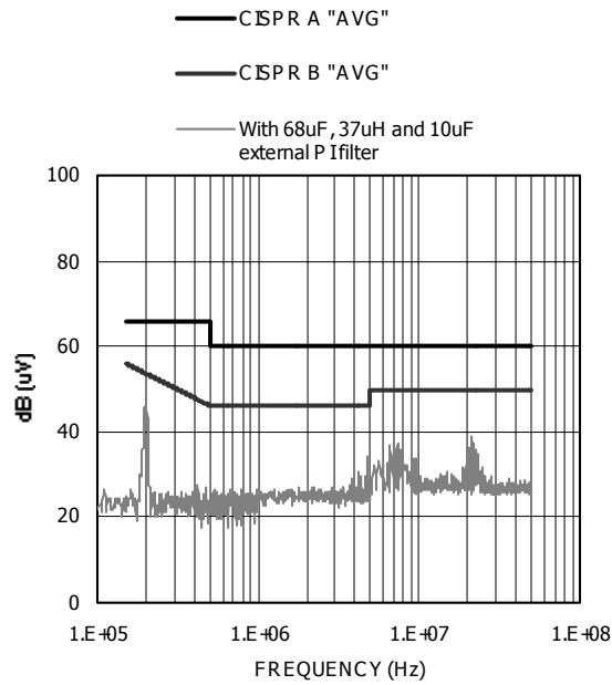
Figure 18. Conducted Emissions at V_{IN} = 48V with External PI Filter, 20A load, with input PI Filter
