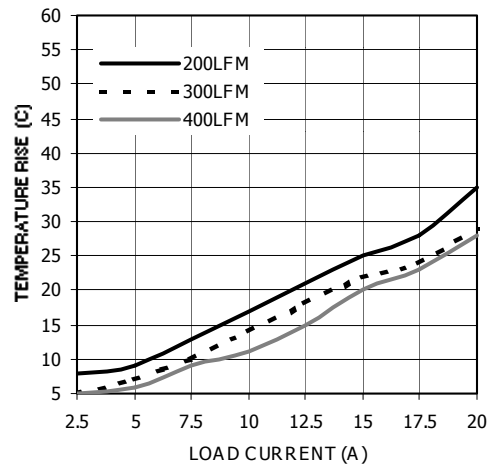
Figure 12. Q6 Case (Hottest component on board) Temperature Rise at 48Vin with 200LFM, 300LFM and 400LFM of Airflow
