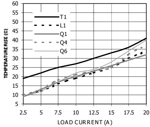
Figure 11. T1 and L1 Core and Q1, Q4, and Q6 Case Temperature Rise at 72Vin with 200LFM of Airflow
