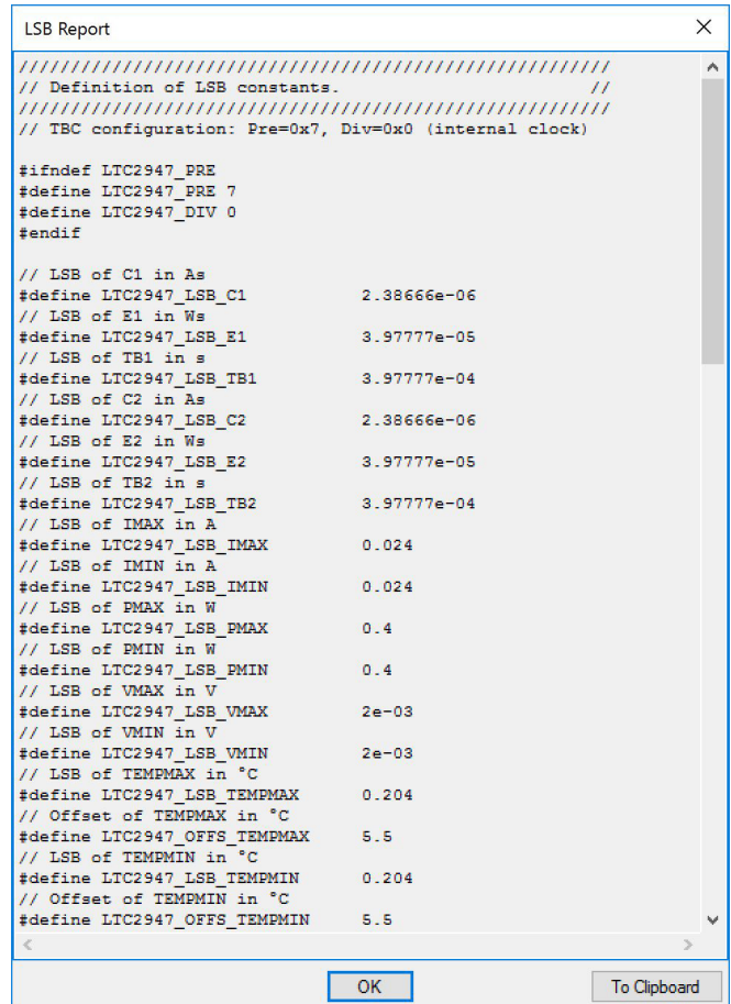
Figure 55. LSB Report
