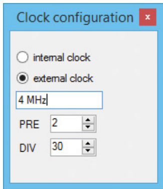
Figure 54. TBC Calculator
