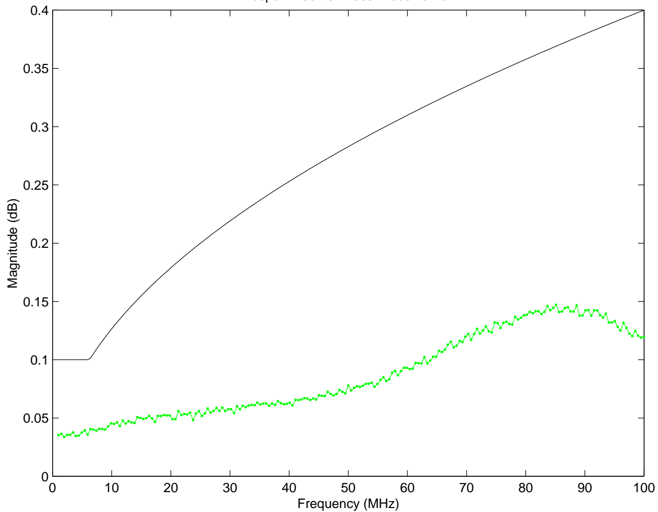
Midspan Insertion Loss: Receive Pair
