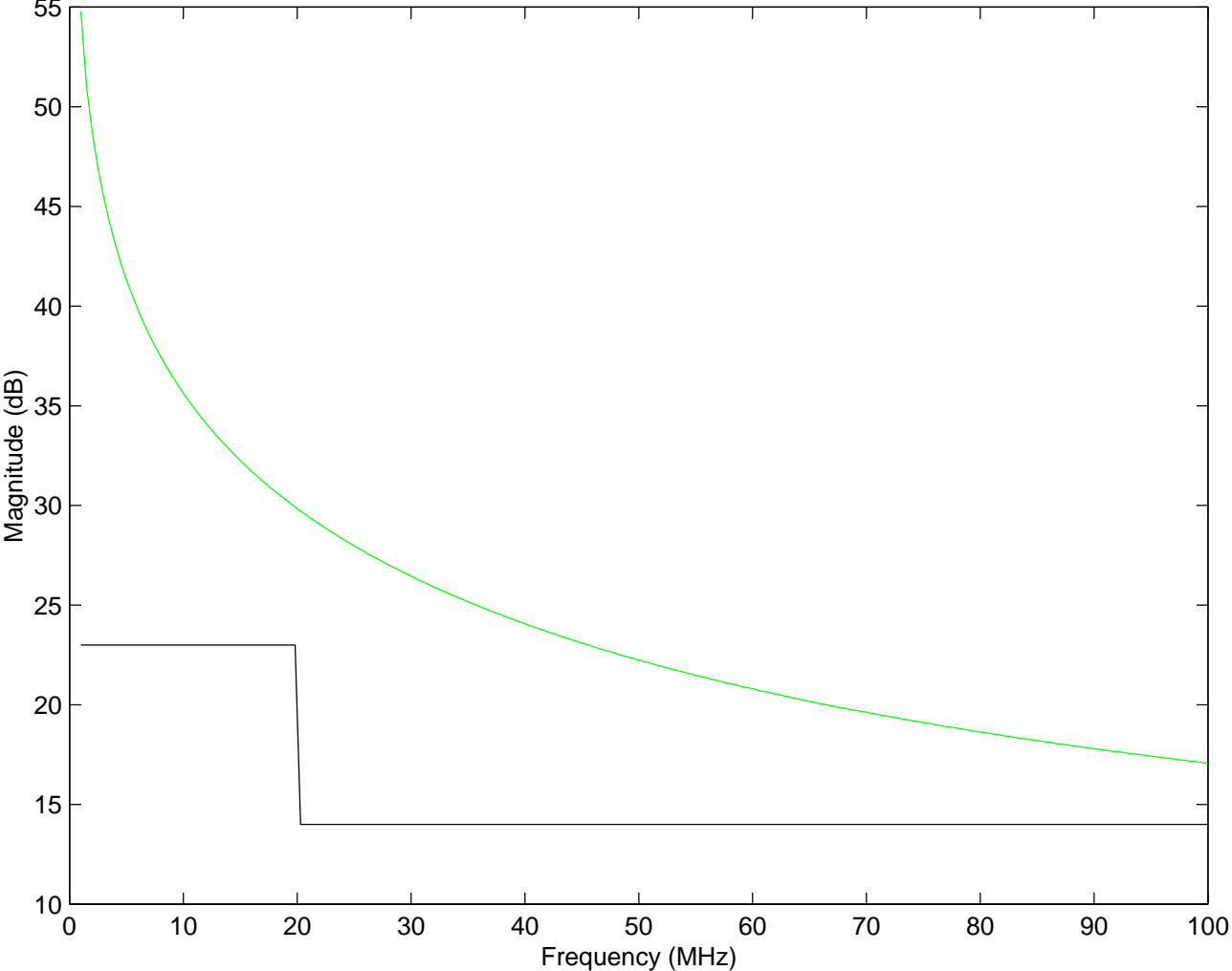
Midspan Return Loss: Receive Pair
