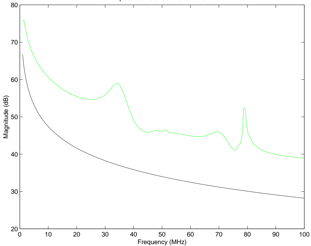
Impedance Balance: Transmit Pair
