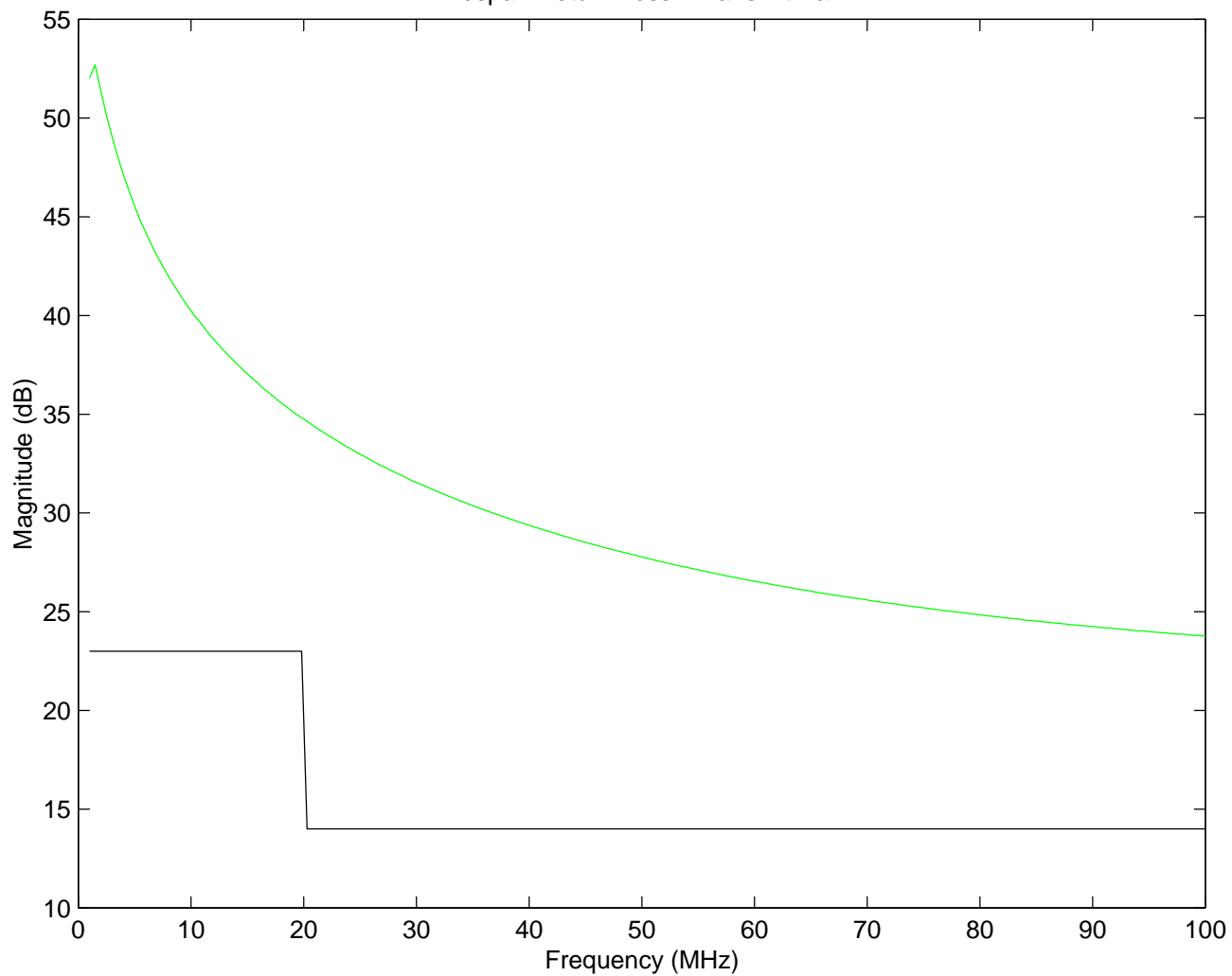
Midspan Return Loss: Transmit Pair
