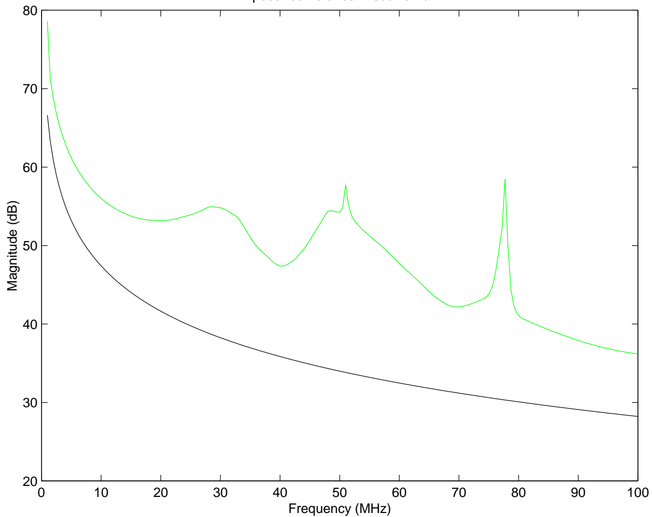
Impedance Balance: Receive Pair
