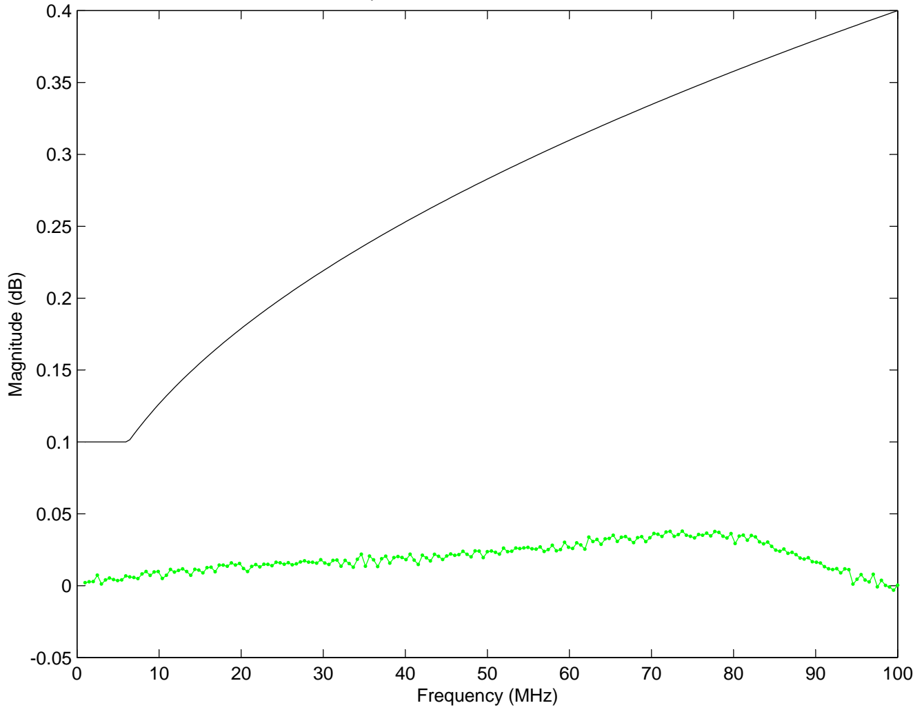
Midspan Insertion Loss: Transmit Pair
