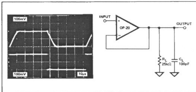
SMALL-SIGNAL TRANSIENT RESPONSE
