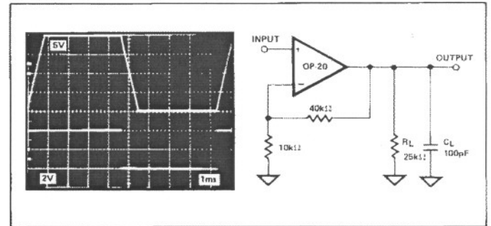
LARGE-SIGNAL TRANSIENT RESPONSE
