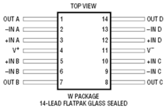
Figure B.2. Package drawing (for reference only). This figure was extracted from Linear Technology RH1014M Quad Precision Operational Amplifier Datasheet.
