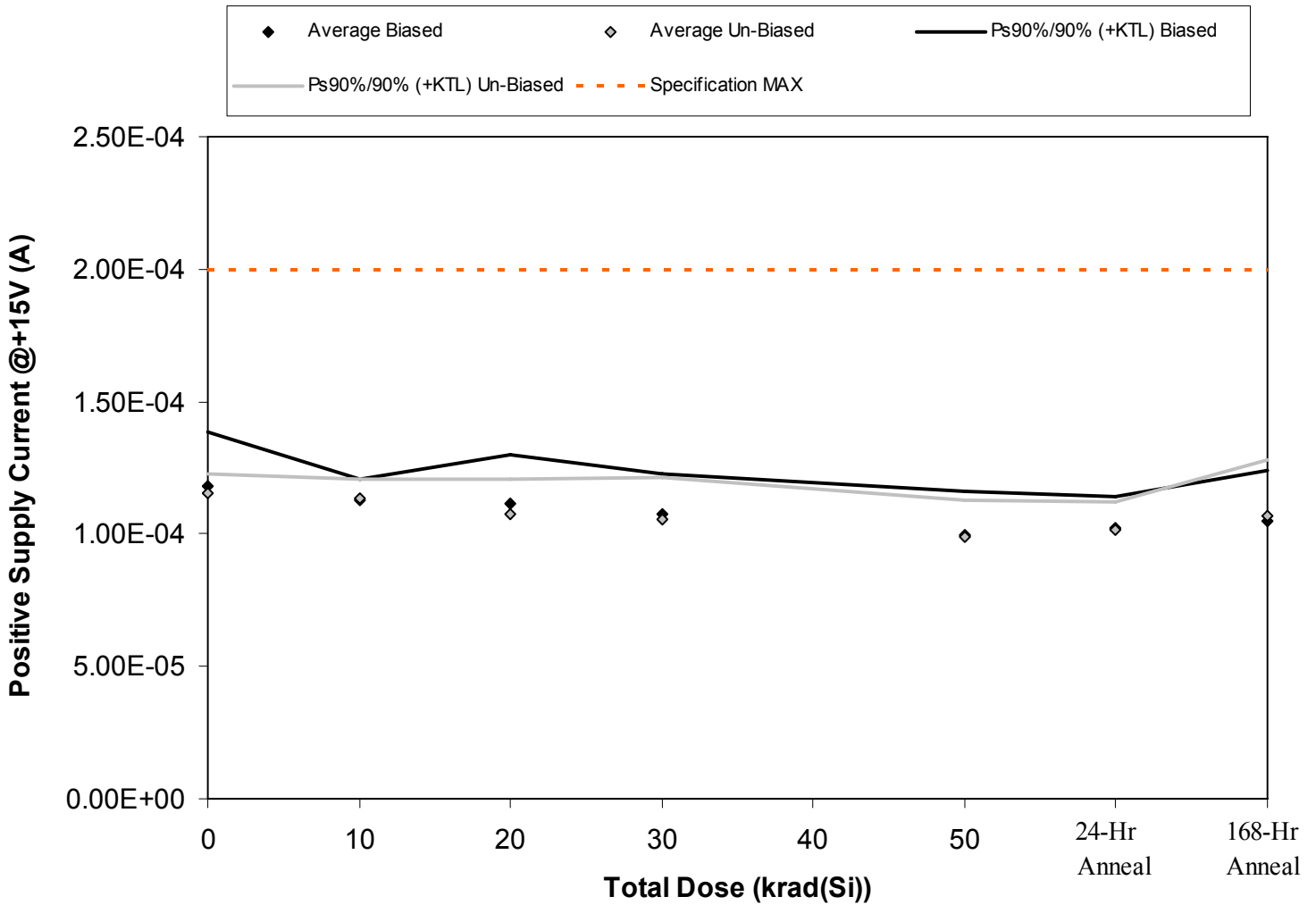
Figure 5.33. Plot of Positive Supply Current @+15V (A) versus total dose. The solid diamonds are the average of the measured data points for the samples irradiated under electrical bias while the shaded diamonds are the average of the measured data points for the samples irradiated with all pins tied to ground. The black lines (solid and/or dashed) are the average of the data points after application of the KTL statistics on the samples irradiated under electrical bias while the gray lines (solid and/or dashed) are the average of the data points after application of the KTL statistics on the samples irradiated in the unbiased condition. The red dotted line(s) are the pre- and/or post-irradiation minimum and/or maximum specification value as defined in the datasheet and/or test plan.
