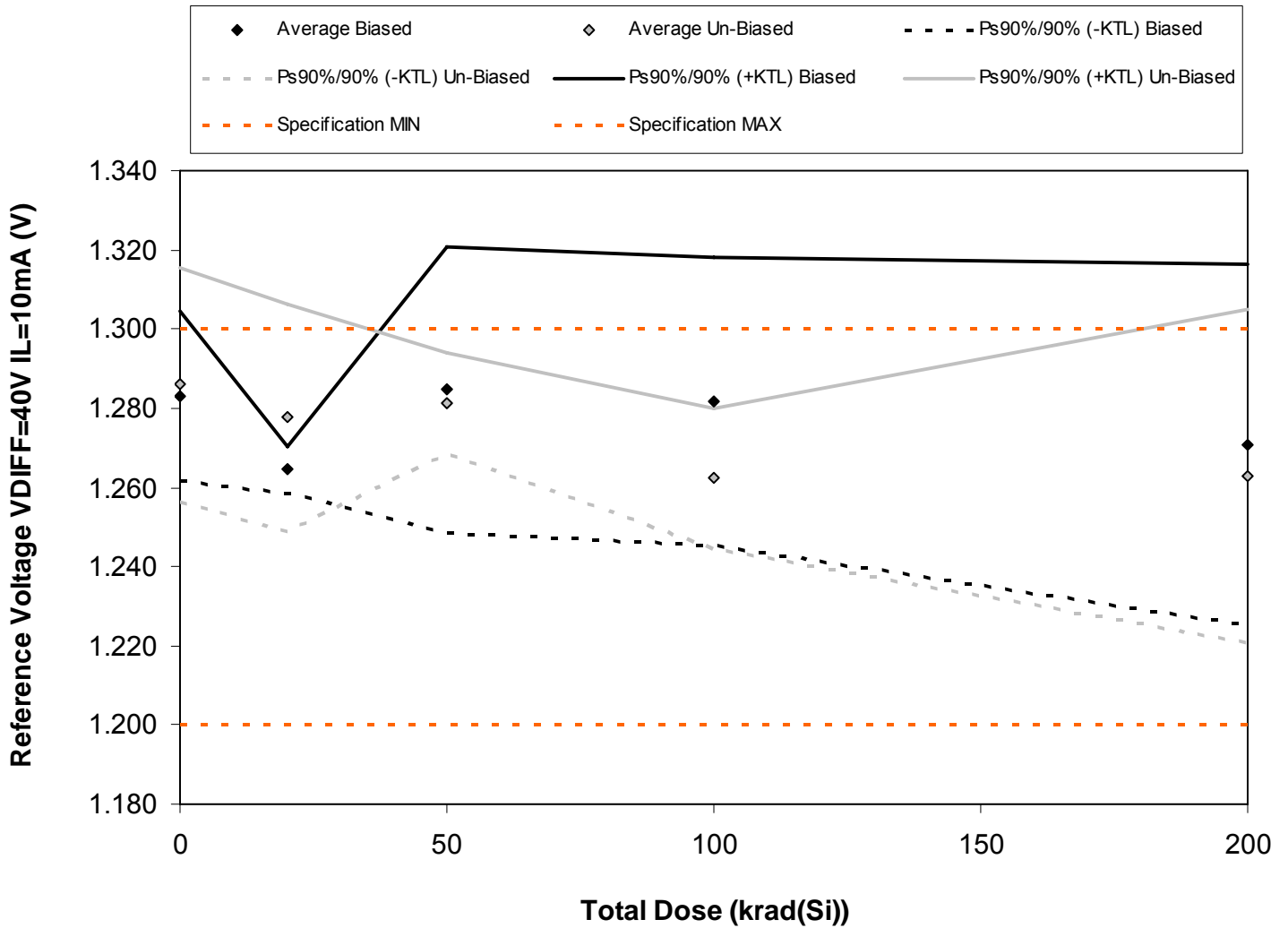
Figure 5.2. Plot of Reference Voltage VDIFF=40V IL=10mA (V) versus total dose. The solid diamonds are the average of the measured data points for the samples irradiated under electrical bias while the shaded diamonds are the average of the measured data points for the samples irradiated with all pins tied to ground. The black lines (solid and/or dashed) are the average of the data points after application of the KTL statistics on the samples irradiated under electrical bias while the gray lines (solid and/or dashed) are the average of the data points after application of the KTL statistics on the samples irradiated in the unbiased condition. The red dotted line(s) are the pre- and/or post-irradiation minimum and/or maximum specification value as defined in the datasheet and/or test plan.
