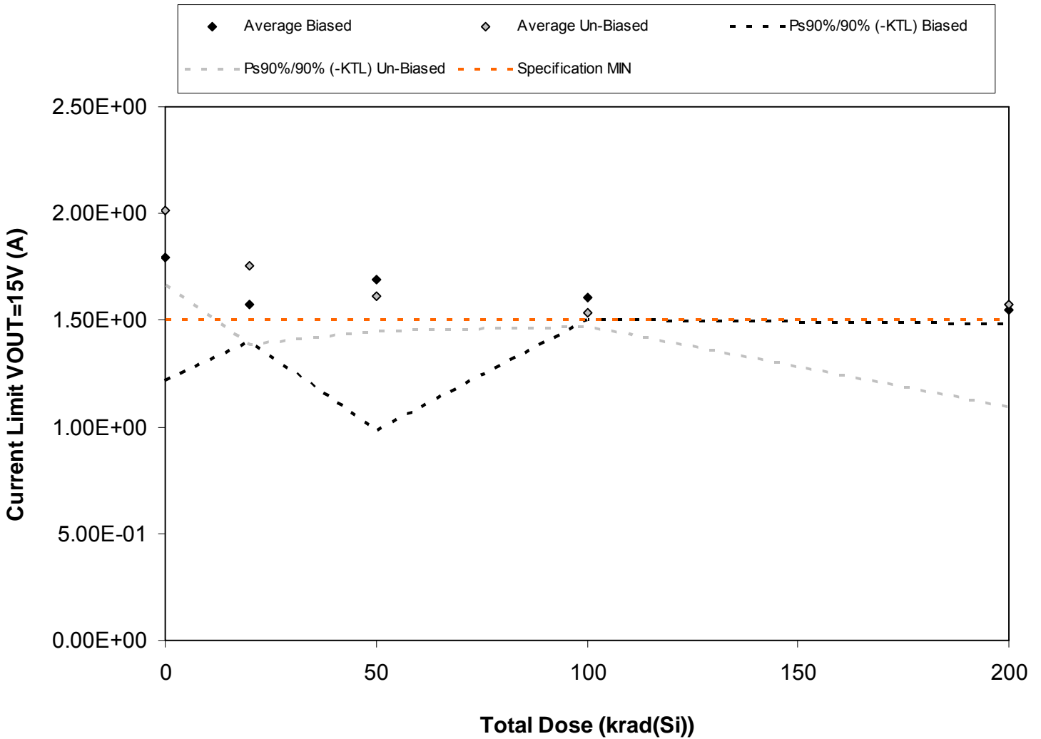
Figure 5.14. Plot of Current Limit VOUT=15V (A) versus total dose. The solid diamonds are the average of the measured data points for the samples irradiated under electrical bias while the shaded diamonds are the average of the measured data points for the samples irradiated with all pins tied to ground. The black lines (solid and/or dashed) are the average of the data points after application of the KTL statistics on the samples irradiated under electrical bias while the gray lines (solid and/or dashed) are the average of the data points after application of the KTL statistics on the samples irradiated in the unbiased condition. The red dotted line(s) are the pre- and/or post-irradiation minimum and/or maximum specification value as defined in the datasheet and/or test plan.
