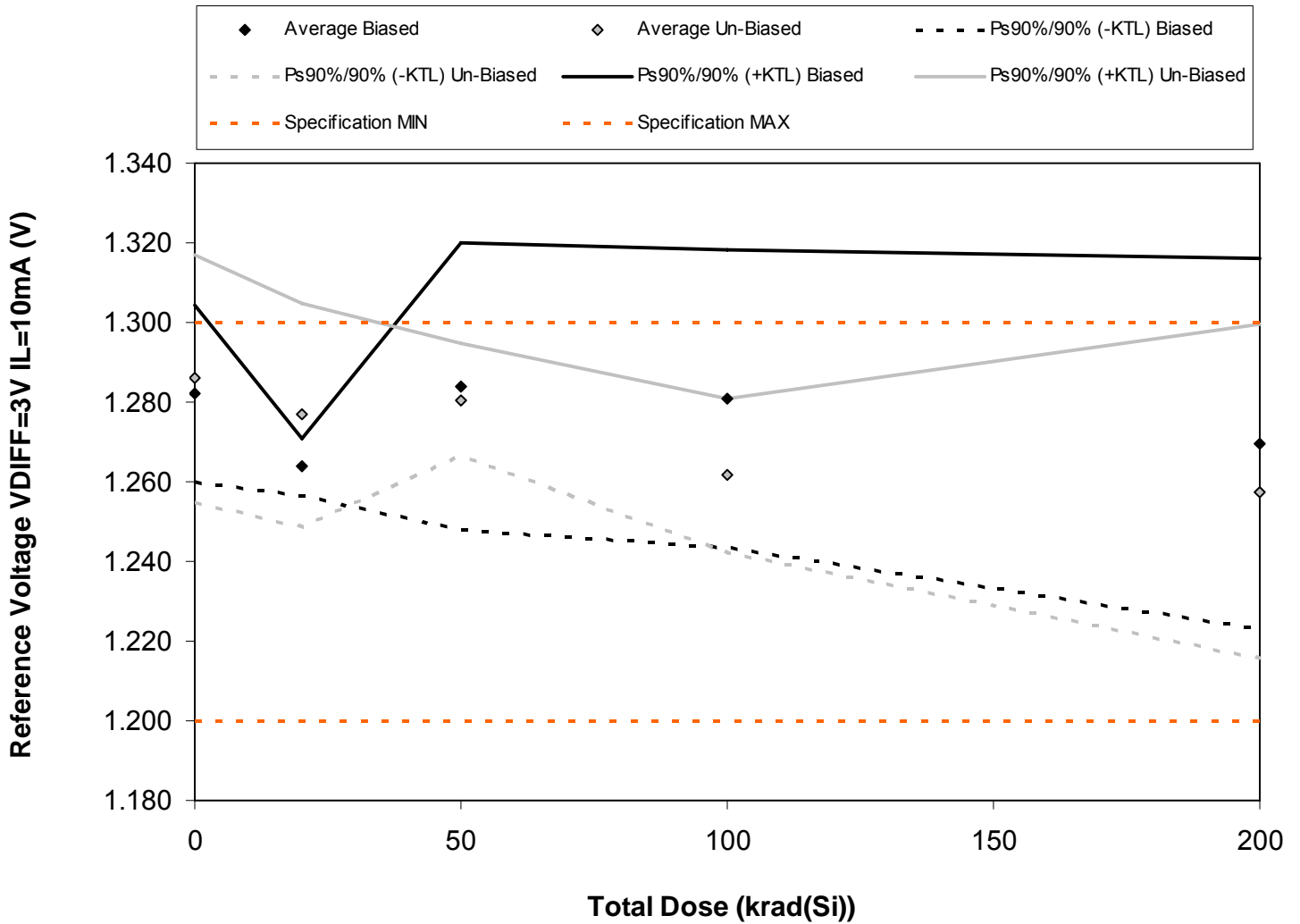
Figure 5.1. Plot of Reference Voltage VDIFF=3V IL=10mA (V) versus total dose. The solid diamonds are the average of the measured data points for the samples irradiated under electrical bias while the shaded diamonds are the average of the measured data points for the samples irradiated with all pins tied to ground. The black lines (solid and/or dashed) are the average of the data points after application of the KTL statistics on the samples irradiated under electrical bias while the gray lines (solid and/or dashed) are the average of the data points after application of the KTL statistics on the samples irradiated in the unbiased condition. The red dotted line(s) are the pre- and/or post-irradiation minimum and/or maximum specification value as defined in the datasheet and/or test plan.
