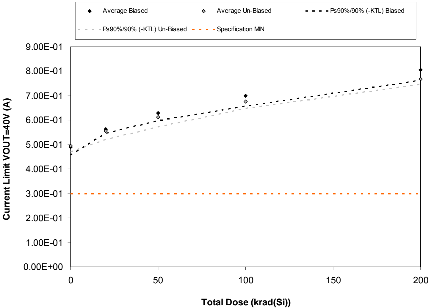
Figure 5.15. Plot of Current Limit VOUT=40V (A) versus total dose. The solid diamonds are the average of the measured data points for the samples irradiated under electrical bias while the shaded diamonds are the average of the measured data points for the samples irradiated with all pins tied to ground. The black lines (solid and/or dashed) are the average of the data points after application of the KTL statistics on the samples irradiated under electrical bias while the gray lines (solid and/or dashed) are the average of the data points after application of the KTL statistics on the samples irradiated in the unbiased condition. The red dotted line(s) are the pre- and/or post-irradiation minimum and/or maximum specification value as defined in the datasheet and/or test plan.
