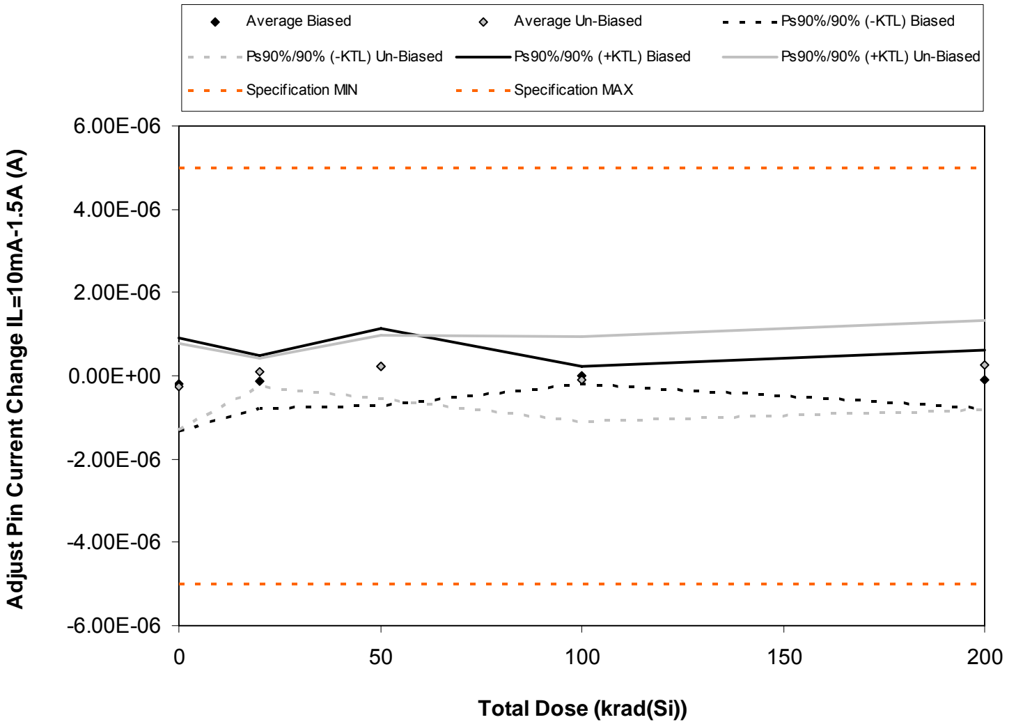
Figure 5.11. Plot of Adjust Pin Current Change IL=10mA-1.5A (A) versus total dose. The solid diamonds are the average of the measured data points for the samples irradiated under electrical bias while the shaded diamonds are the average of the measured data points for the samples irradiated with all pins tied to ground. The black lines (solid and/or dashed) are the average of the data points after application of the KTL statistics on the samples irradiated under electrical bias while the gray lines (solid and/or dashed) are the average of the data points after application of the KTL statistics on the samples irradiated in the unbiased condition. The red dotted line(s) are the pre- and/or post-irradiation minimum and/or maximum specification value as defined in the datasheet and/or test plan.
