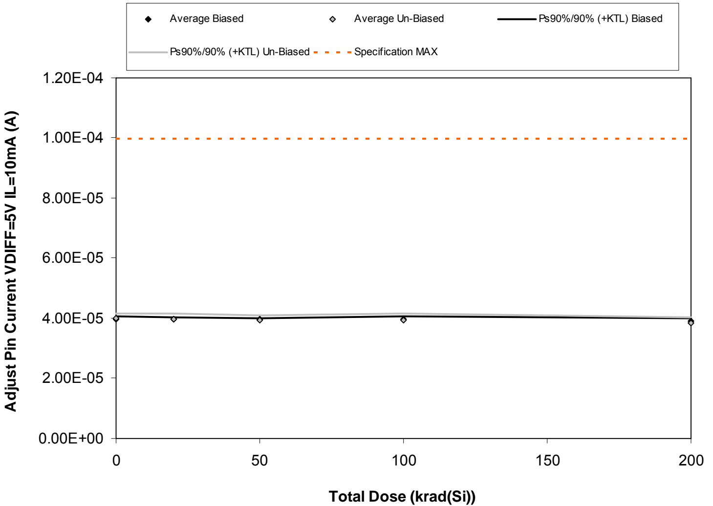
Figure 5.9. Plot of Adjust Pin Current VDIFF=5V IL=10mA (A) versus total dose. The solid diamonds are the average of the measured data points for the samples irradiated under electrical bias while the shaded diamonds are the average of the measured data points for the samples irradiated with all pins tied to ground. The black lines (solid and/or dashed) are the average of the data points after application of the KTL statistics on the samples irradiated under electrical bias while the gray lines (solid and/or dashed) are the average of the data points after application of the KTL statistics on the samples irradiated in the unbiased condition. The red dotted line(s) are the pre- and/or post-irradiation minimum and/or maximum specification value as defined in the datasheet and/or test plan.
