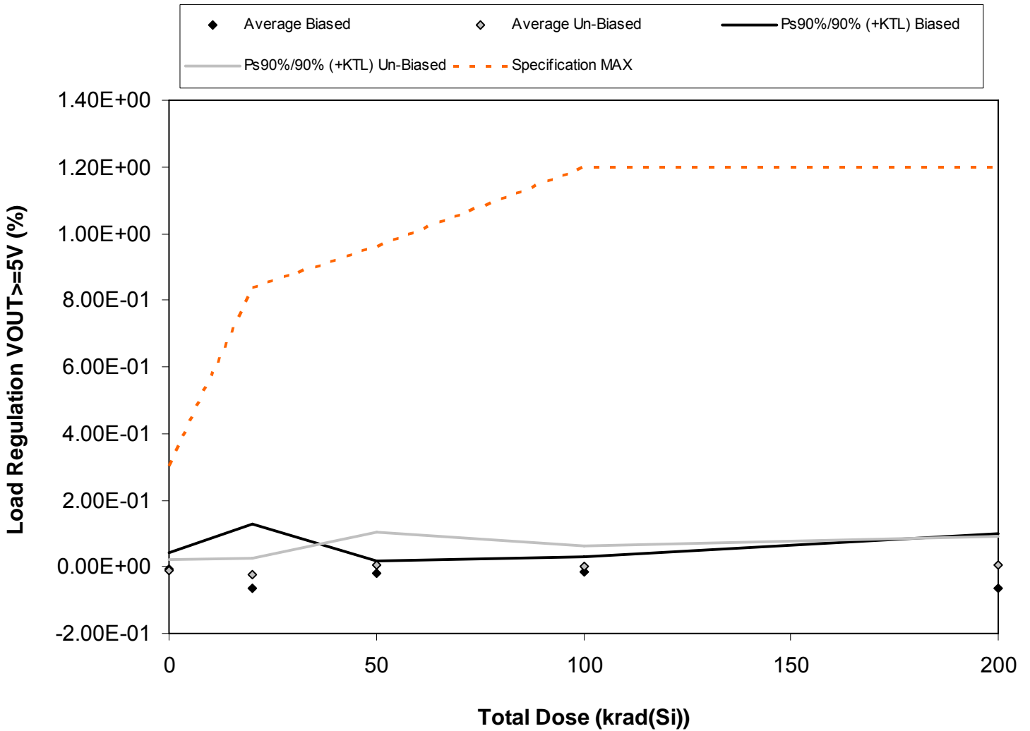
Figure 5.7. Plot of Load Regulation VOUT >= 5V (%) versus total dose. The solid diamonds are the average of the measured data points for the samples irradiated under electrical bias while the shaded diamonds are the average of the measured data points for the samples irradiated with all pins tied to ground. The black lines (solid and/or dashed) are the average of the data points after application of the KTL statistics on the samples irradiated under electrical bias while the gray lines (solid and/or dashed) are the average of the data points after application of the KTL statistics on the samples irradiated in the unbiased condition. The red dotted line(s) are the pre- and/or post-irradiation minimum and/or maximum specification value as defined in the datasheet and/or test plan.
