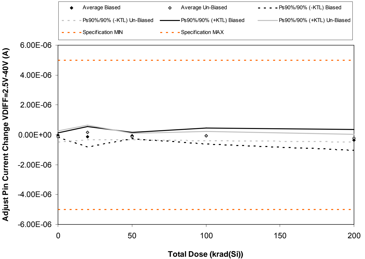
Figure 5.12. Plot of Adjust Pin Current Change VDIFF=2.5V-40V (A) versus total dose. The solid diamonds are the average of the measured data points for the samples irradiated under electrical bias while the shaded diamonds are the average of the measured data points for the samples irradiated with all pins tied to ground. The black lines (solid and/or dashed) are the average of the data points after application of the KTL statistics on the samples irradiated under electrical bias while the gray lines (solid and/or dashed) are the average of the data points after application of the KTL statistics on the samples irradiated in the unbiased condition. The red dotted line(s) are the pre- and/or post-irradiation minimum and/or maximum specification value as defined in the datasheet and/or test plan.
