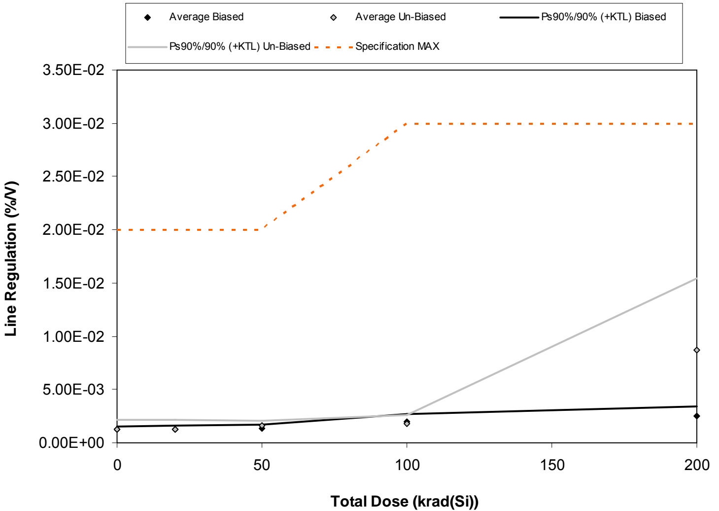
Figure 5.5. Plot of Line Regulation (%/V) versus total dose. The solid diamonds are the average of the measured data points for the samples irradiated under electrical bias while the shaded diamonds are the average of the measured data points for the samples irradiated with all pins tied to ground. The black lines (solid and/or dashed) are the average of the data points after application of the KTL statistics on the samples irradiated under electrical bias while the gray lines (solid and/or dashed) are the average of the data points after application of the KTL statistics on the samples irradiated in the unbiased condition. The red dotted line(s) are the pre- and/or post-irradiation minimum and/or maximum specification value as defined in the datasheet and/or test plan.
