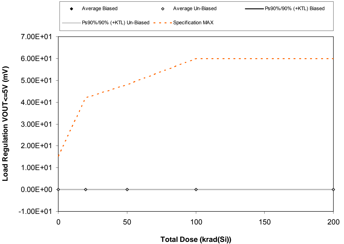
Figure 5.6. Plot of Load Regulation VOUT<=5V (mV) versus total dose. The solid diamonds are the average of the measured data points for the samples irradiated under electrical bias while the shaded diamonds are the average of the measured data points for the samples irradiated with all pins tied to ground. The black lines (solid and/or dashed) are the average of the data points after application of the KTL statistics on the samples irradiated under electrical bias while the gray lines (solid and/or dashed) are the average of the data points after application of the KTL statistics on the samples irradiated in the unbiased condition. The red dotted line(s) are the pre- and/or post-irradiation minimum and/or maximum specification value as defined in the datasheet and/or test plan.
