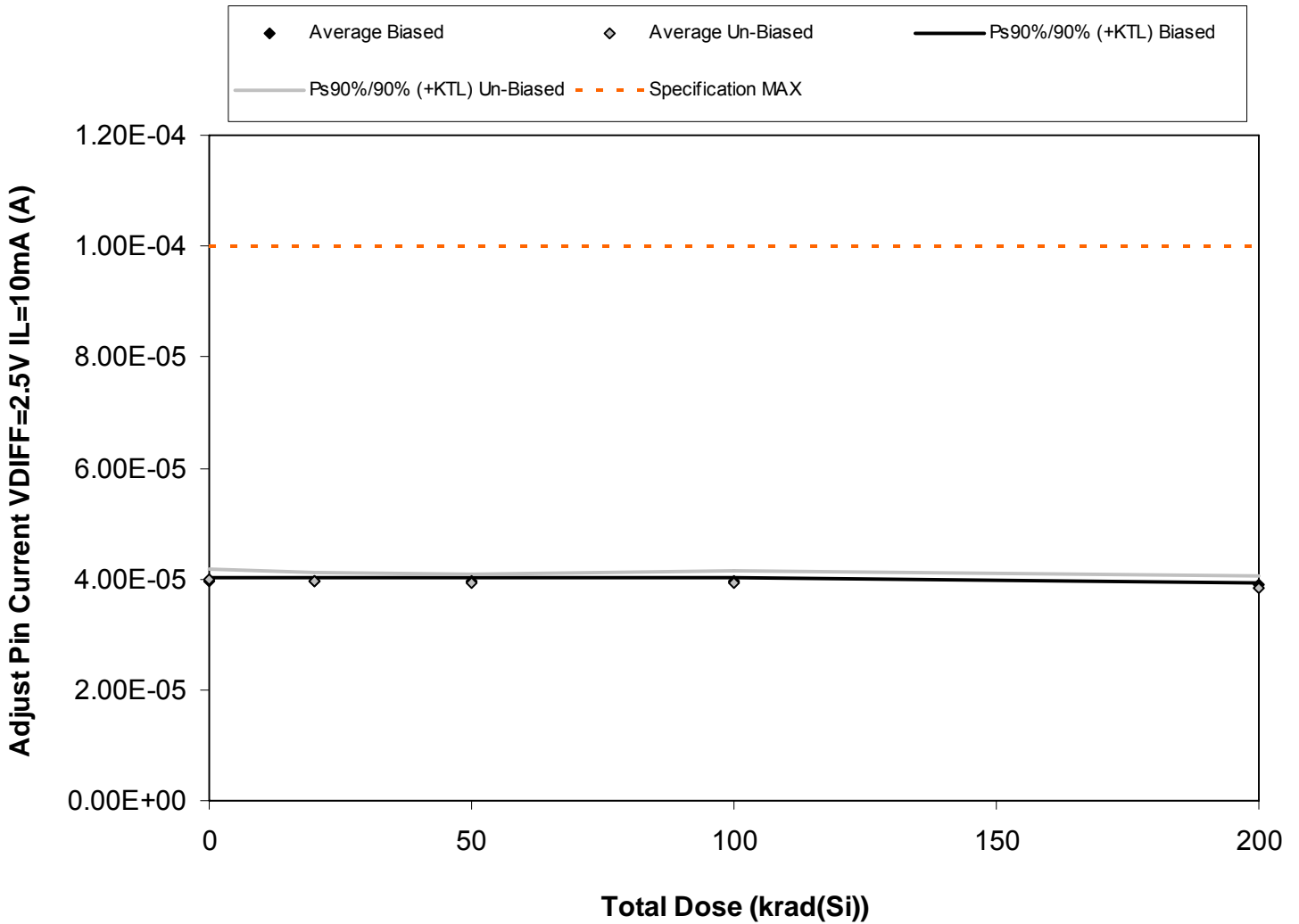
Figure 5.8. Plot of Adjust Pin Current VDIFF=2.5V IL=10mA (A) versus total dose. The solid diamonds are the average of the measured data points for the samples irradiated under electrical bias while the shaded diamonds are the average of the measured data points for the samples irradiated with all pins tied to ground. The black lines (solid and/or dashed) are the average of the data points after application of the KTL statistics on the samples irradiated under electrical bias while the gray lines (solid and/or dashed) are the average of the data points after application of the KTL statistics on the samples irradiated in the unbiased condition. The red dotted line(s) are the pre- and/or post-irradiation minimum and/or maximum specification value as defined in the datasheet and/or test plan.
