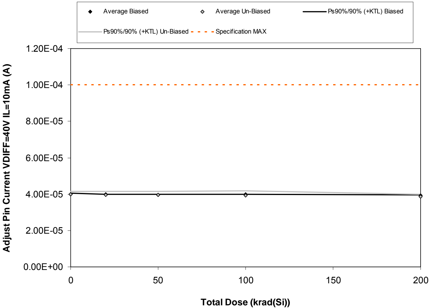
Figure 5.10. Plot of Adjust Pin Current VDIFF=40V IL=10mA (A) versus total dose. The solid diamonds are the average of the measured data points for the samples irradiated under electrical bias while the shaded diamonds are the average of the measured data points for the samples irradiated with all pins tied to ground. The black lines (solid and/or dashed) are the average of the data points after application of the KTL statistics on the samples irradiated under electrical bias while the gray lines (solid and/or dashed) are the average of the data points after application of the KTL statistics on the samples irradiated in the unbiased condition. The red dotted line(s) are the pre- and/or post-irradiation minimum and/or maximum specification value as defined in the datasheet and/or test plan.
