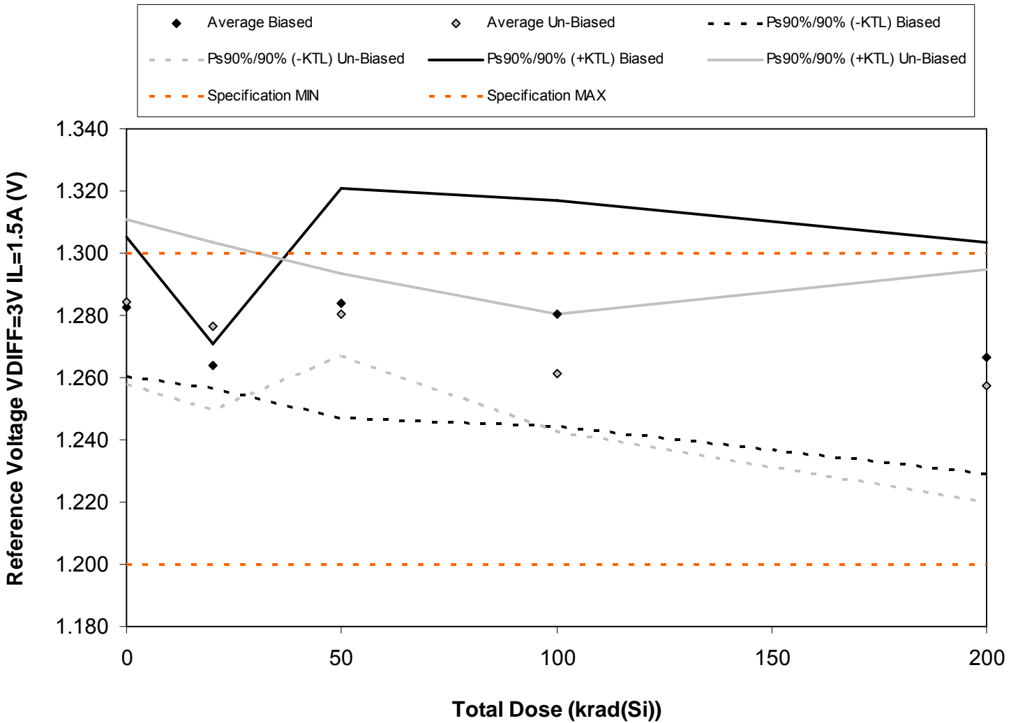
Figure 5.3. Plot of Reference Voltage V_{DIFF}=3V I_L=1.5A (V) versus total dose. The solid diamonds are the average of the measured data points for the samples irradiated under electrical bias while the shaded diamonds are the average of the measured data points for the samples irradiated with all pins tied to ground. The black lines (solid and/or dashed) are the average of the data points after application of the KTL statistics on the samples irradiated under electrical bias while the gray lines (solid and/or dashed) are the average of the data points after application of the KTL statistics on the samples irradiated in the unbiased condition. The red dotted line(s) are the pre- and/or post-irradiation minimum and/or maximum specification value as defined in the datasheet and/or test plan.
