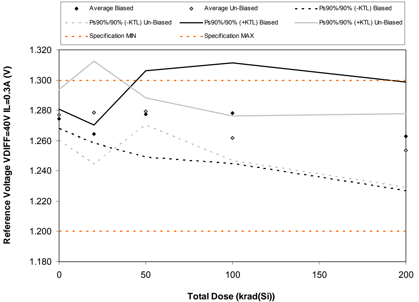
Figure 5.4. Plot of Reference Voltage V_{DIFF}=40V I_L=0.3A (V) versus total dose. The solid diamonds are the average of the measured data points for the samples irradiated under electrical bias while the shaded diamonds are the average of the measured data points for the samples irradiated with all pins tied to ground. The black lines (solid and/or dashed) are the average of the data points after application of the KTL statistics on the samples irradiated under electrical bias while the gray lines (solid and/or dashed) are the average of the data points after application of the KTL statistics on the samples irradiated in the unbiased condition. The red dotted line(s) are the pre- and/or post-irradiation minimum and/or maximum specification value as defined in the datasheet and/or test plan.
