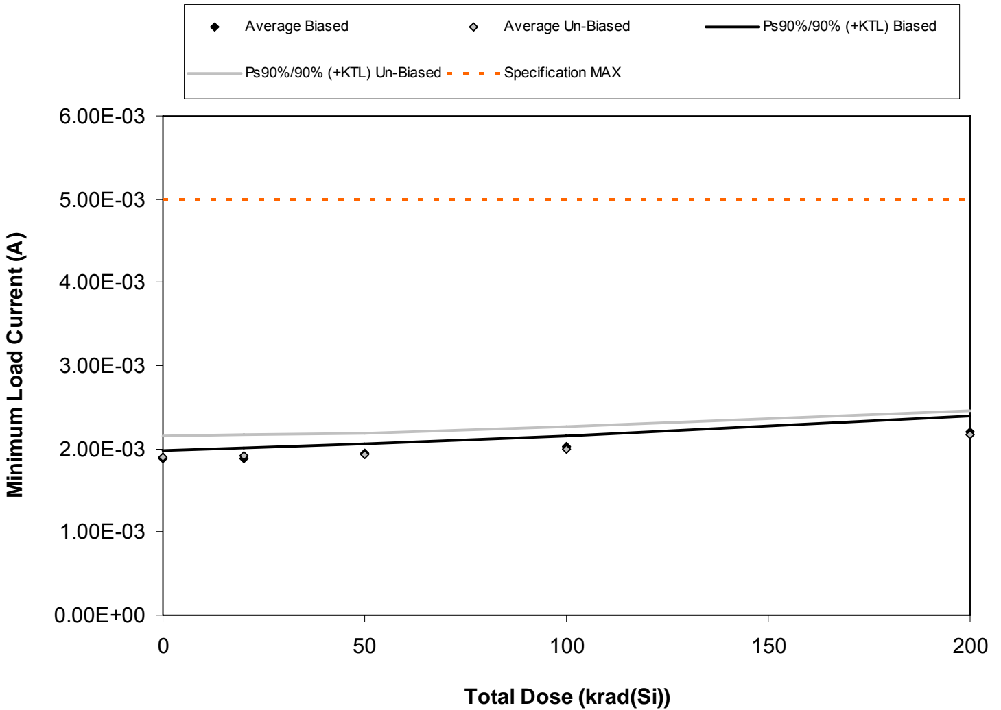
Figure 5.13. Plot of Minimum Load Current (A) versus total dose. The solid diamonds are the average of the measured data points for the samples irradiated under electrical bias while the shaded diamonds are the average of the measured data points for the samples irradiated with all pins tied to ground. The black lines (solid and/or dashed) are the average of the data points after application of the KTL statistics on the samples irradiated under electrical bias while the gray lines (solid and/or dashed) are the average of the data points after application of the KTL statistics on the samples irradiated in the unbiased condition. The red dotted line(s) are the pre- and/or post-irradiation minimum and/or maximum specification value as defined in the datasheet and/or test plan.
