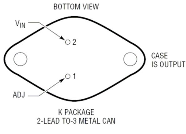
Figure B.2. K package drawing (for reference only). This figure was extracted from the LINEAR TECHNOLOGY CORPORATION RH117 Datasheet.
