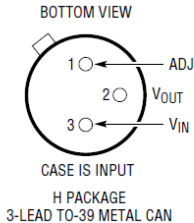
Figure B.2. H package drawing (for reference only). This figure was extracted from the Linear Technology RH137 Datasheet
