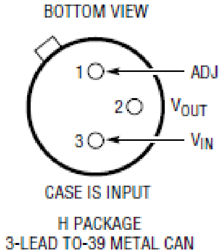
Figure B.2. H package drawing (for reference only). This figure was extracted from Linear Technology RH137 Datasheet Revision C.
