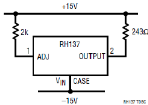
Figure B.1. Irradiation bias circuit. This figure was extracted from Linear Technology RH137 Datasheet Revision C.
