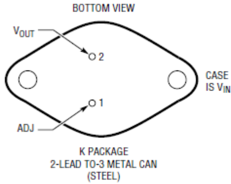
Figure B.2. K package drawing (for reference only). This figure was extracted from Linear Technology RH137 Datasheet.
