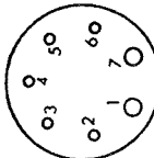
American Small 7 Pin (SM7)
