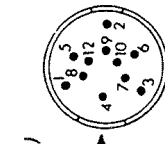
5AA & 7AA (Acorn Valve)
