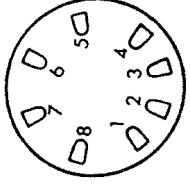
'P' Type Base (8 SC)
