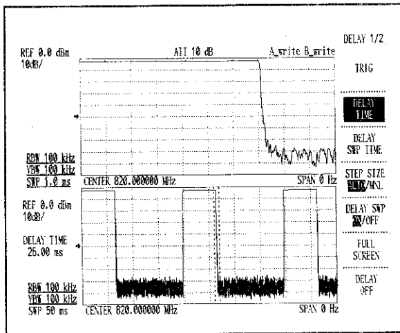
Figure 7 - 24 Split-Screen Display (DELAYED SWEEP ON)
