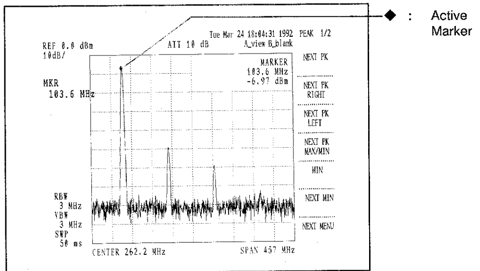
Figure 5.3-6 Peak Search Screen
