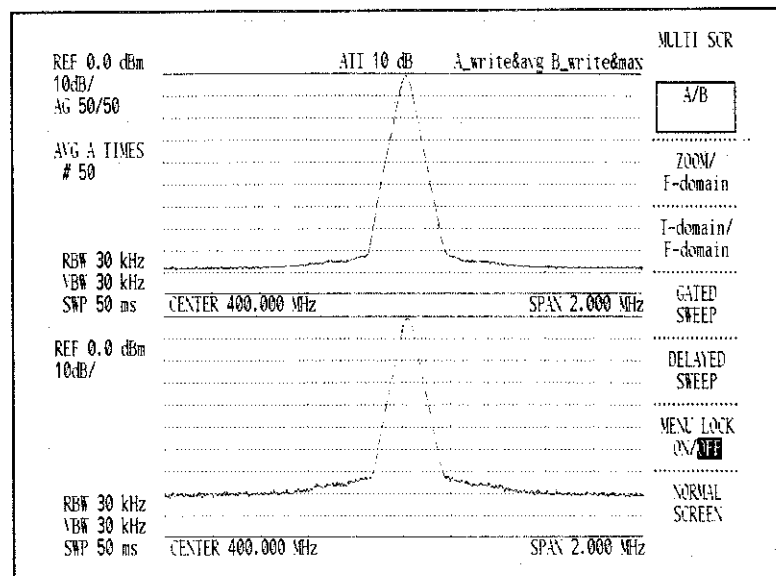
Figure 7 - 1 A/B Mode
