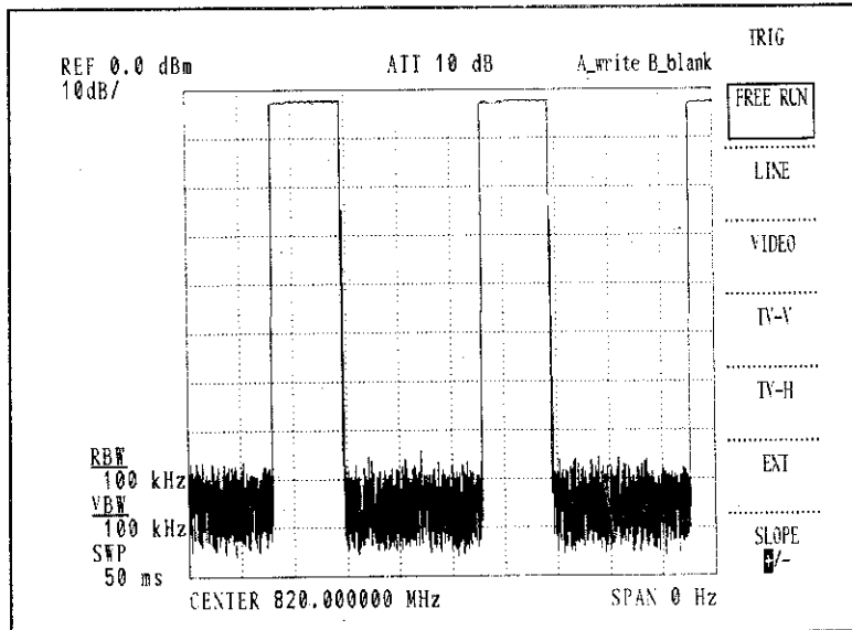
Figure 7 - 26 Full-Screen Display
