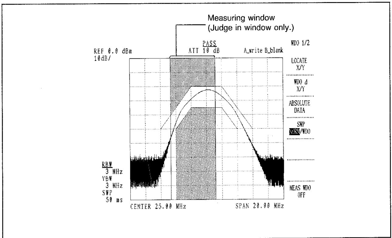
Figure 5.20-3 Judgment Range when Measuring Window is ON
