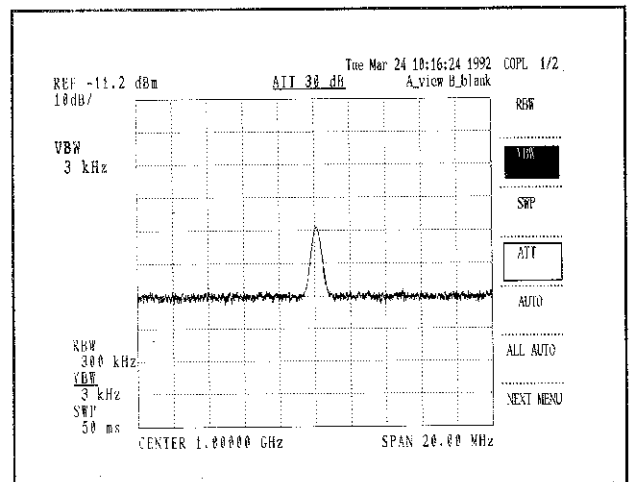
Figure 5.1-8 VBW = 3kHz
