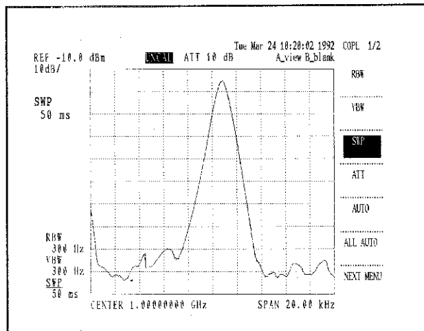
Figure 5.1-10 SWP = 50ms
