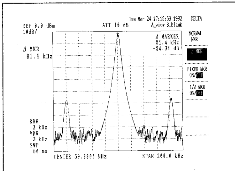
Figure 5.3-2 Delta Marker
