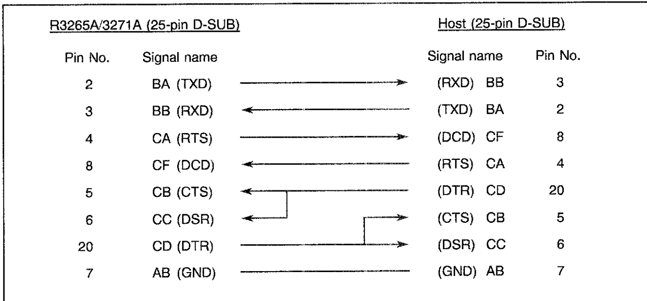
Figure 5.18-3 Cable Connection
