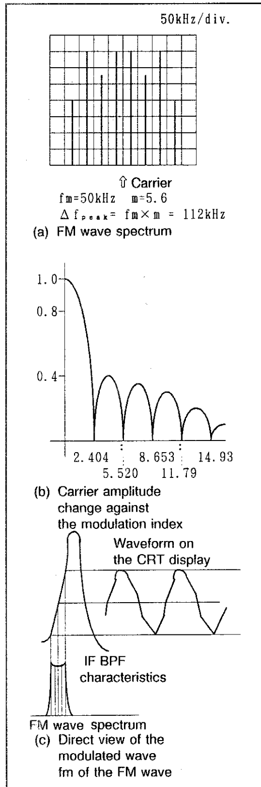
Figure 4-9 Measuring an FM Signal
