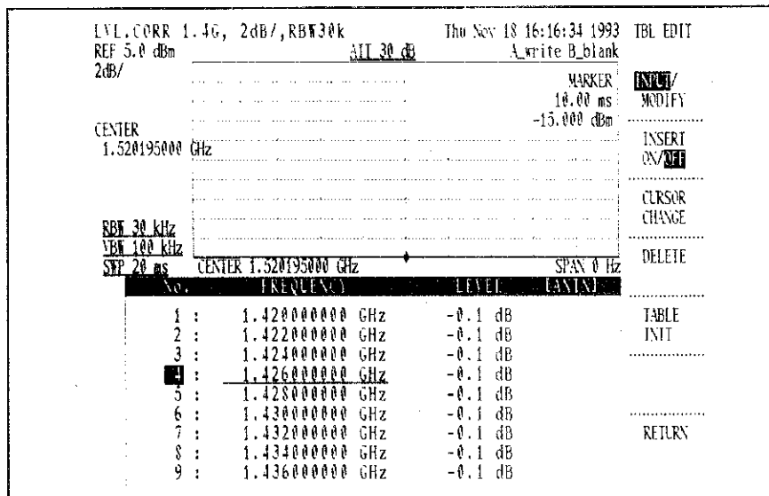
Figure 5.23-2 Checking Calibration Data
