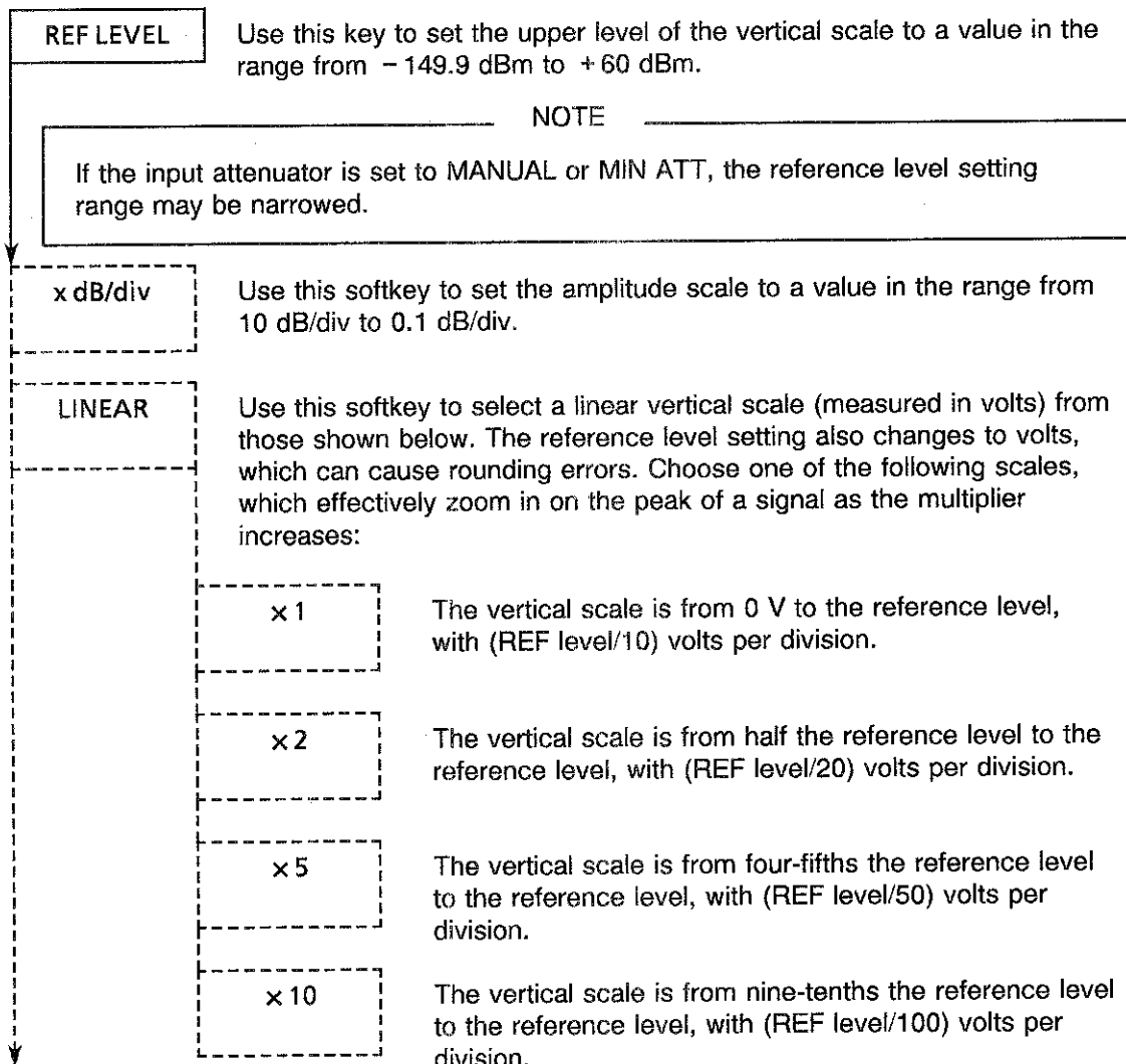
Figure 5.1-5 Reference Level
