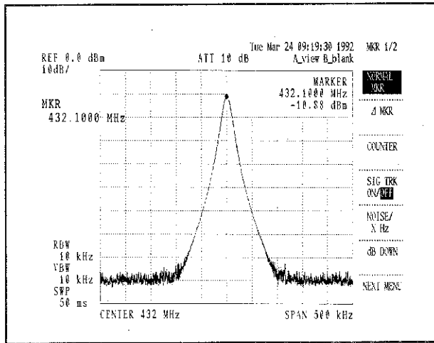
Figure 3-6 Peak Marker
