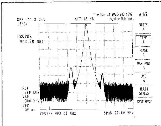
Figure 5.2-3 AVG = None
