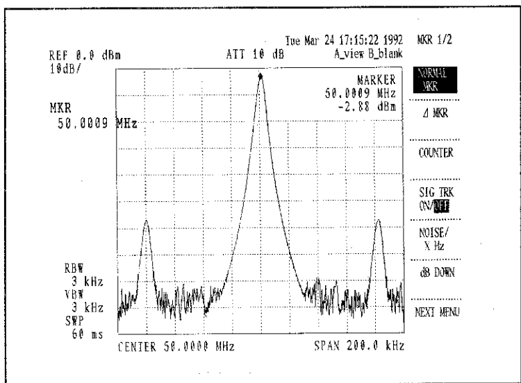
Figure 5.3-1 Normal Marker
