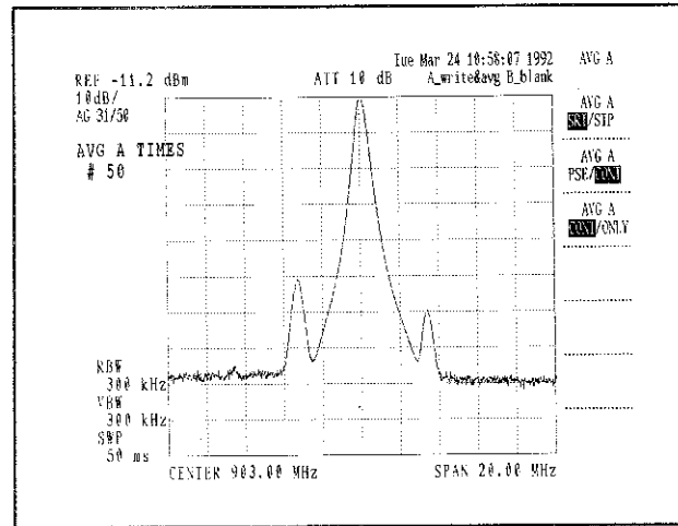
Figure 5.2-4 AVG = 31st
