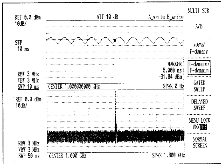
Figure 7 - 9 TIME-domain/F-domain Mode
