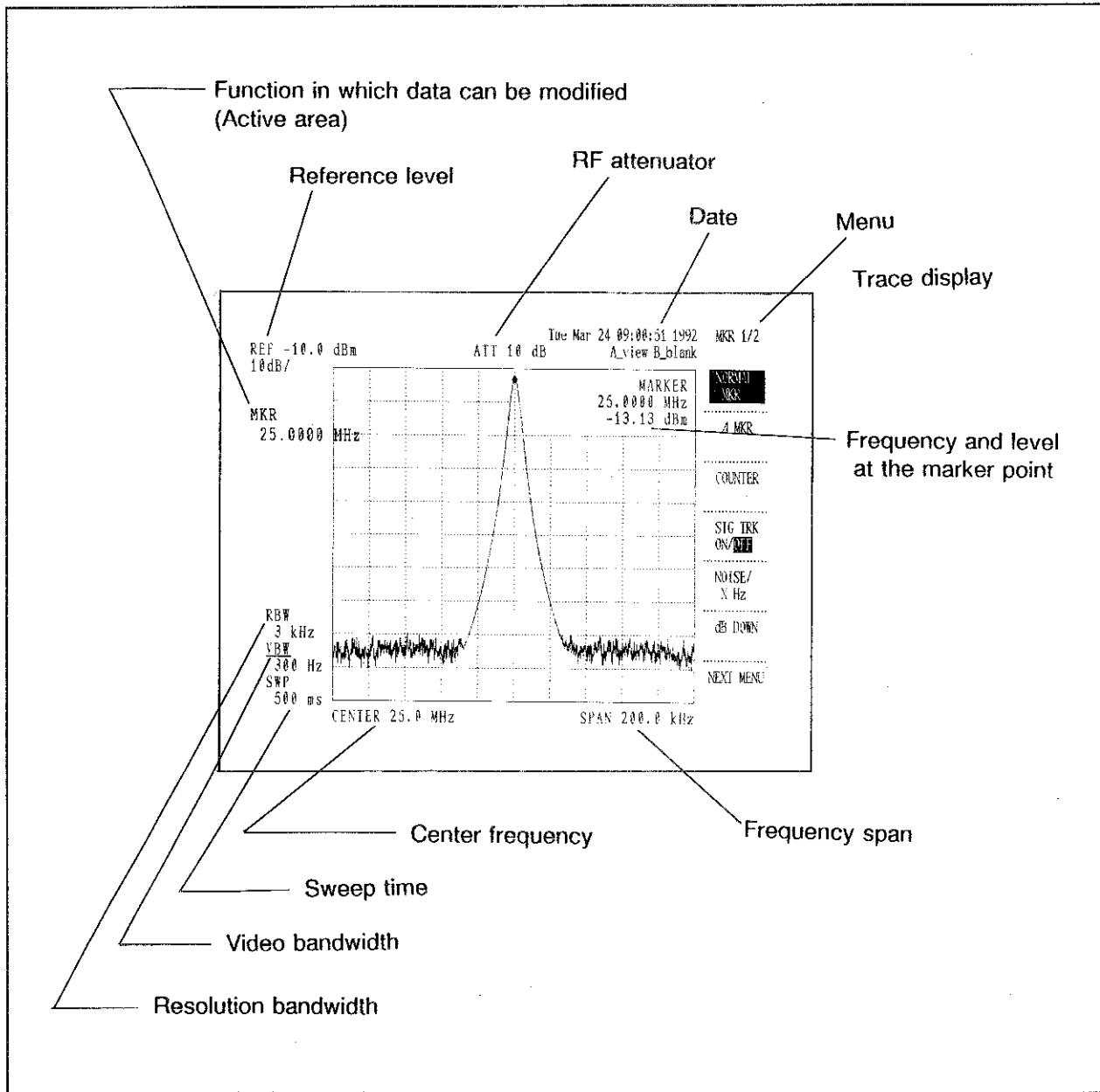
Figure 3-1 Display
