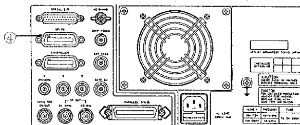
Rear Panel
