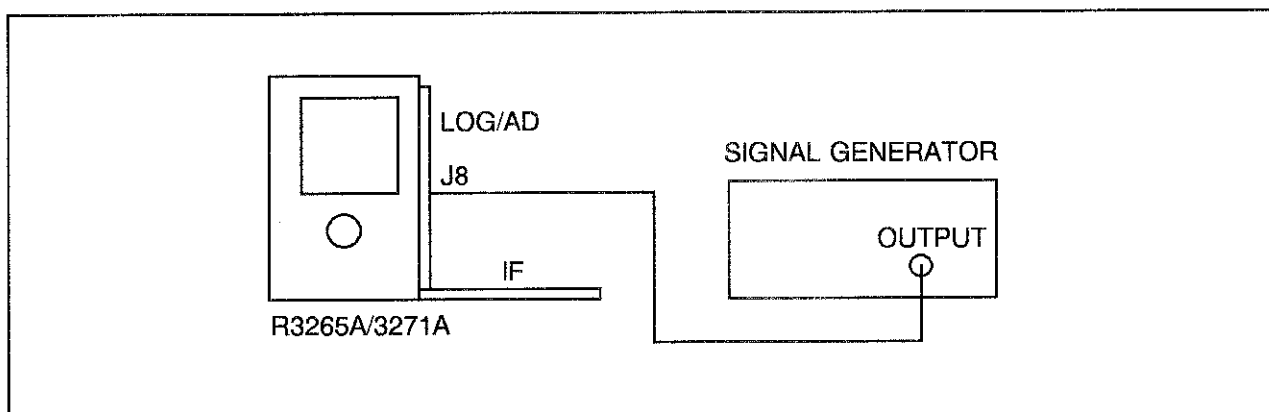
Figure 5-5 Adjustment Setup
