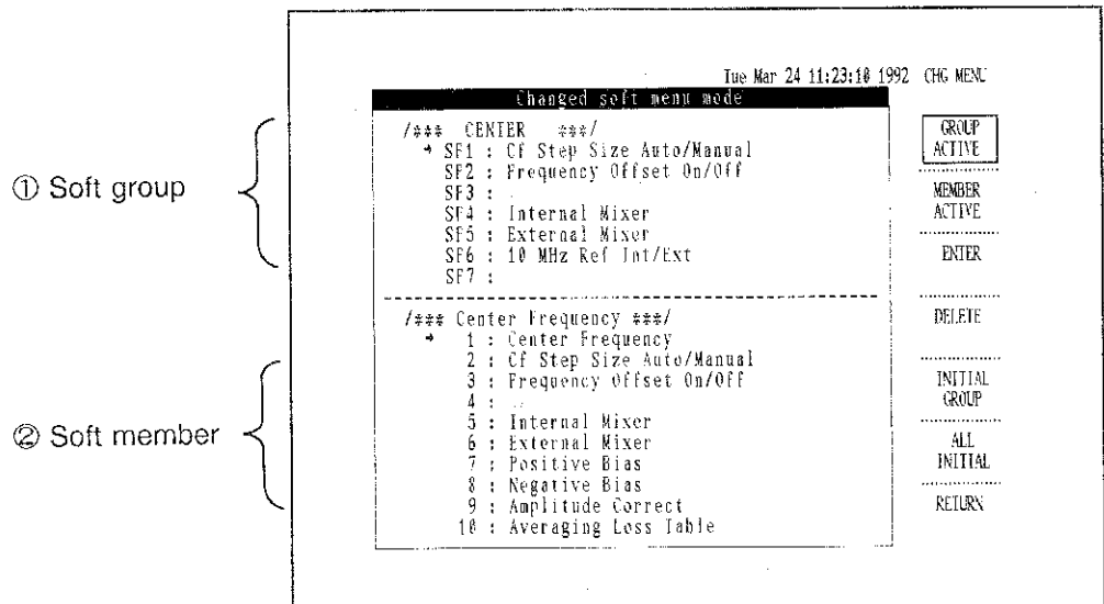
Figure 5.4-1 User-Defined Display
