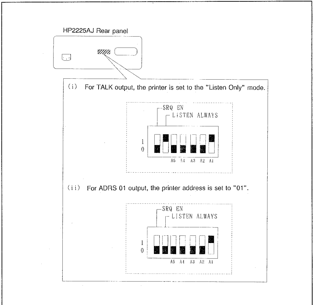
Figure 5.15-2 DIP Switch for Address Setting
