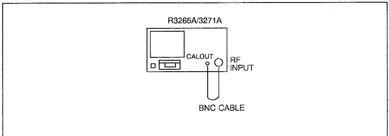
Figure 4-7 Resolution Bandwidth Accuracy/Selectivity Setup
