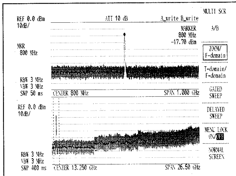
Figure 7 - 5 ZOOM/F-domain Mode
