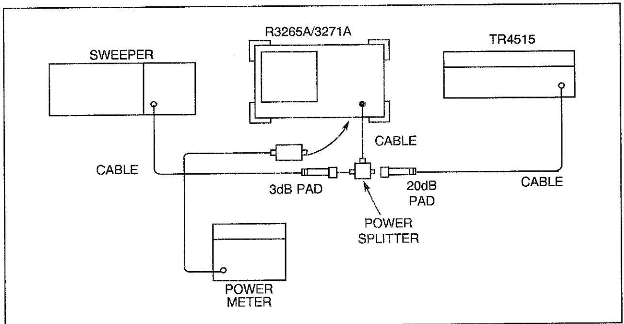
Figure 4-10 Gain Compression Test Setup
