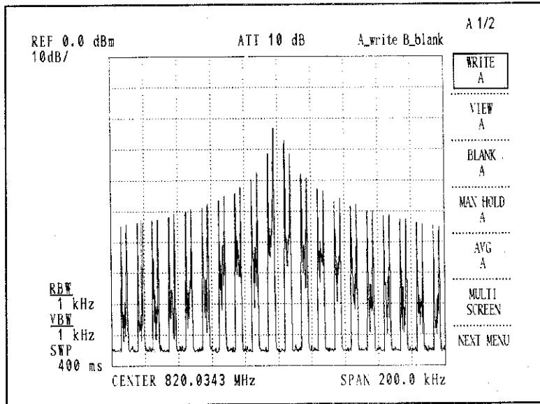
Figure 7 - 18 Full-Screen Display
