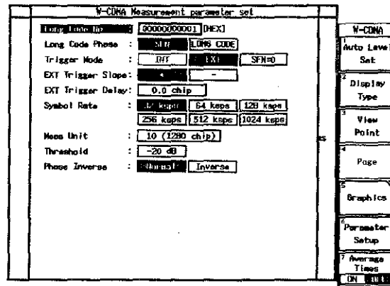
Figure 3-31 Setting of Parameter for W-CDMA Measurement Test
