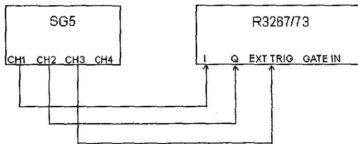
Figure 3-32 Setup of MS Measurement
