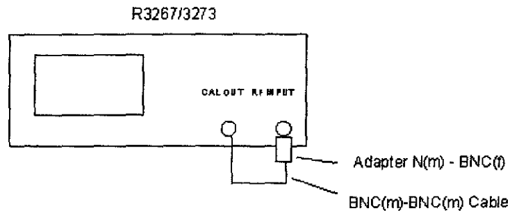
Figure 3-5 Setup of RBW Accuracy and Selectivity Test
