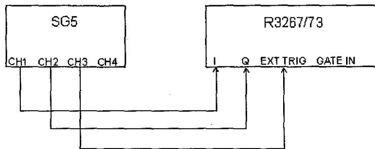
Figure 3-28 Setup of BTS Measurement Test
