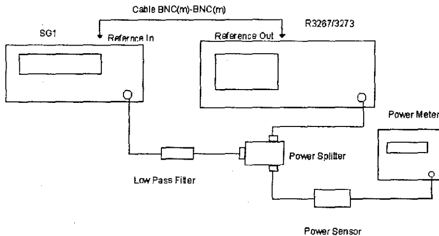
Figure 3-13 Setup of a Second Harmonics Distortion Test
