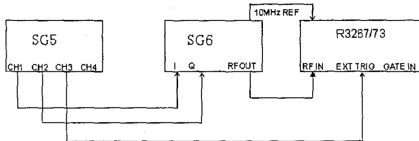
Figure 3-26 Setup of QPSK Measurement Test
