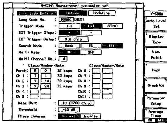
Figure 3-29 Setting of Parameter for W-CDMA Measurement Test
