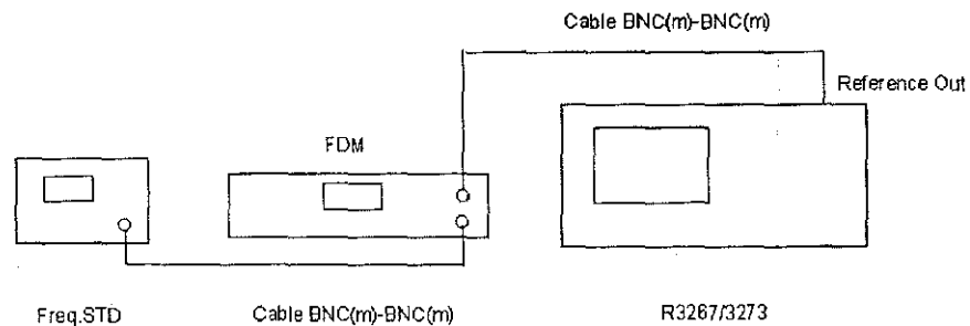
Figure 4-1 Internal Frequency Reference Adjustment Setup
