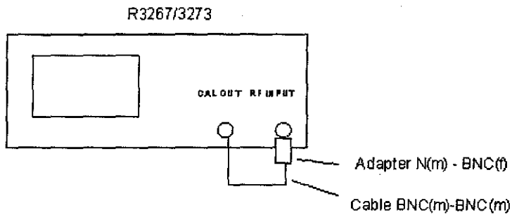
Figure 3-4 Setup of RBW Switching Uncertainty
