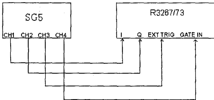
Figure 3-30 Setup of MS Measurement Test
