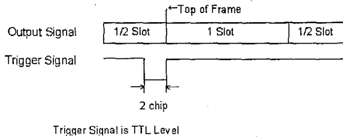
Figure 3-20 Timing Chart of BTS Test Signal
