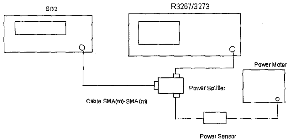
Figure 3-11 Setup of a Image, Multiple, Out of Band Spurious Test
