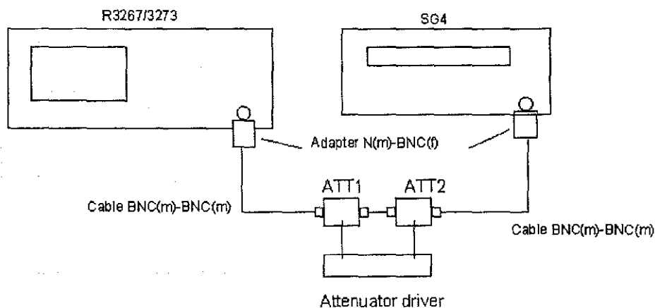
Figure 3-6 Setup of IF Gain Fidelity Test
