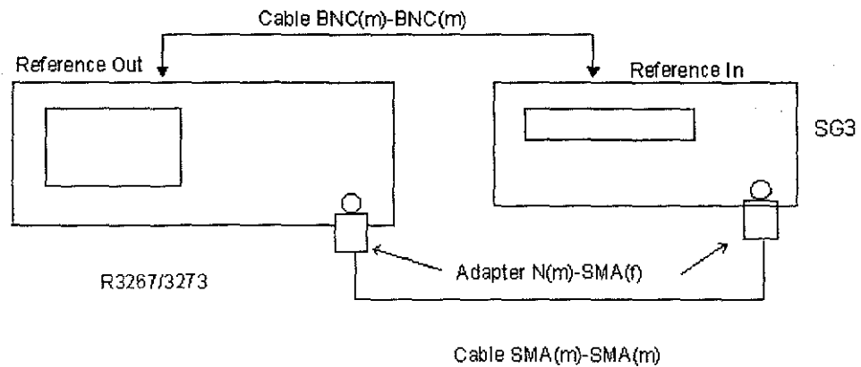
Figure 3-9 Setup of Residual FM Test
