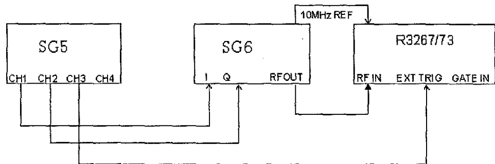
Figure 3-24 Setup of MS Measurement Test
