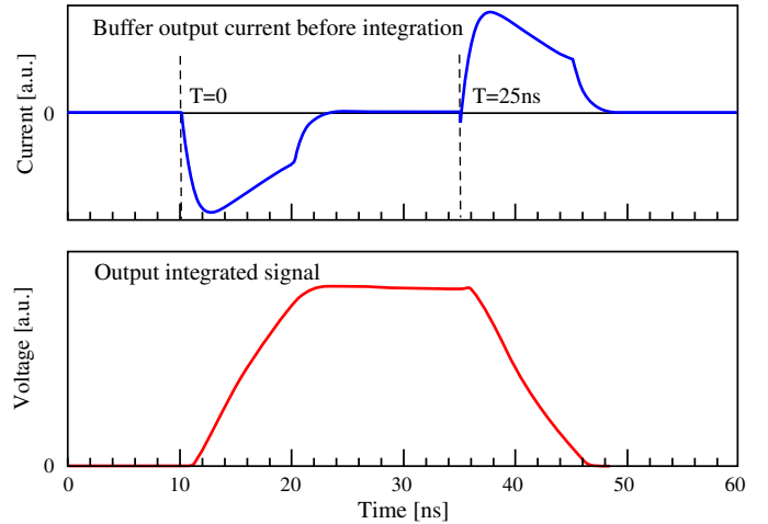
Strobe on the flat top ( \approx 10 ns). Shaping : h(t) = \int [i(t) - i(t+25\text{ns})] dt
