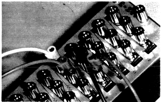
Figure 13 Four-Terminal Connections
