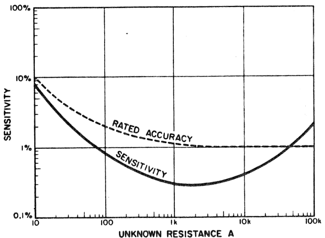
FIGURE 16. BRIDGE SENSITIVITY
