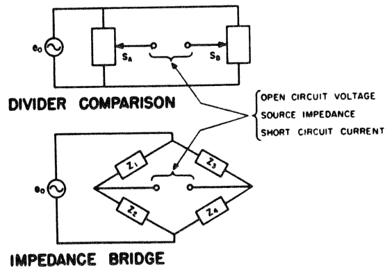
FIGURE 36. OUTPUT CIRCUIT
