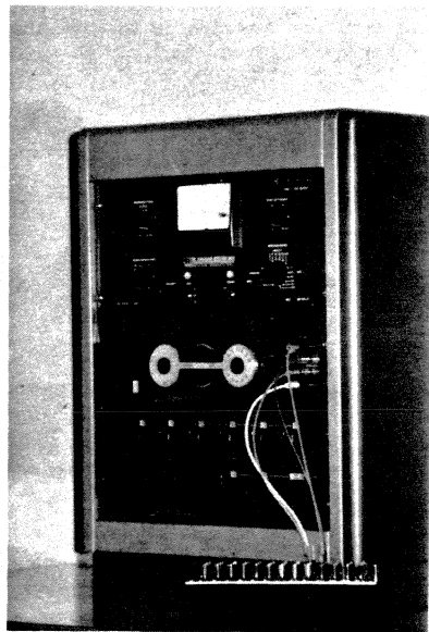
Figure 15 ESI Model 242 Resistance Measuring System
