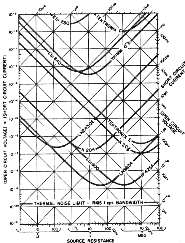
FIGURE 41. DETECTOR COMPARISON
