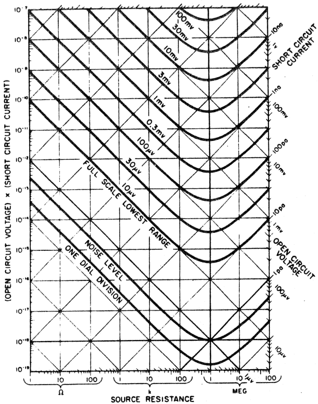
FIGURE 14. DETECTOR CURVES
