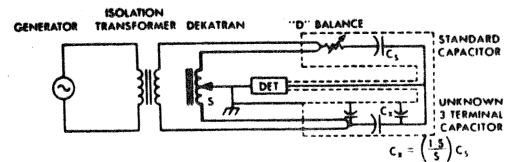
FIGURE 19. CAPACITANCE BRIDGE
