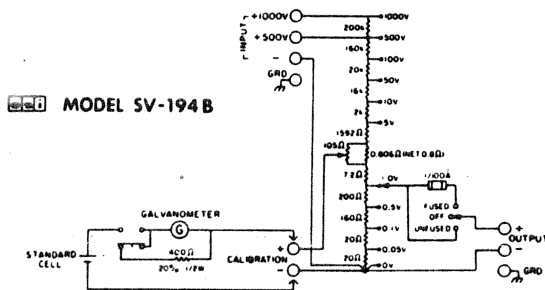
FIGURE 8. CALIBRATOR CIRCUIT
