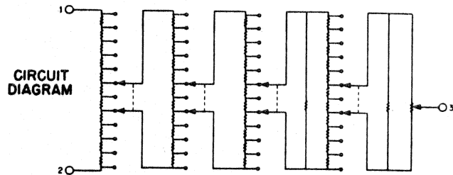
FIGURE 23. KELVIN-VARLEY CIRCUIT
