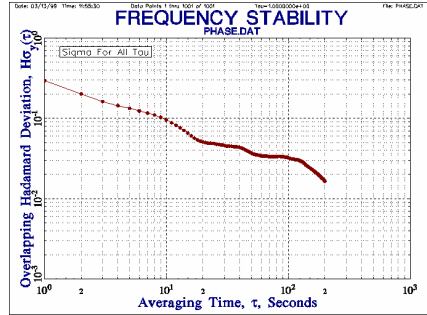
Overlapping Samples
