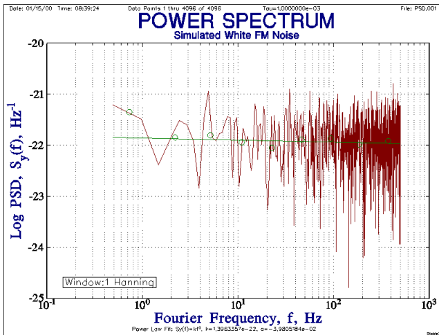
Figure 7.2f S_y(f) Power Spectral Density
