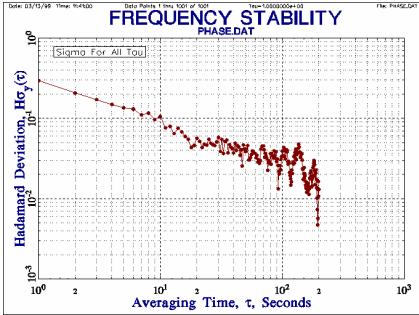
Non-Overlapping Samples
