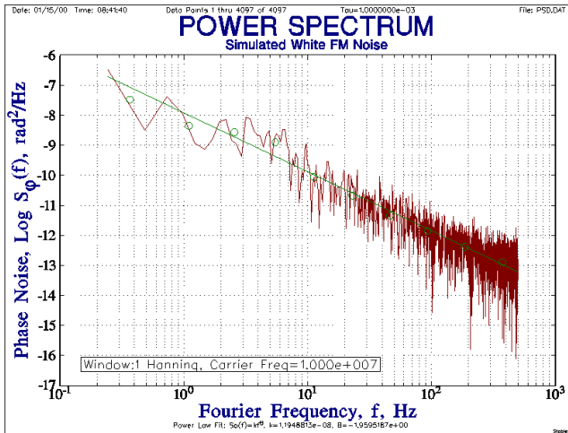
Figure 7.2d S_{\phi}(f) Power Spectral Density
