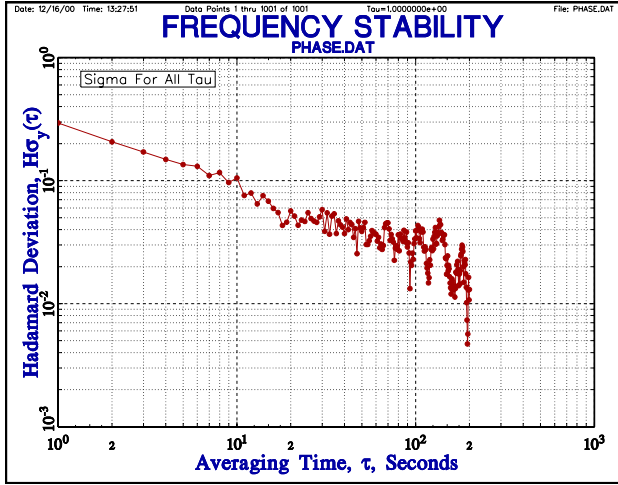
Hadamard Deviation
