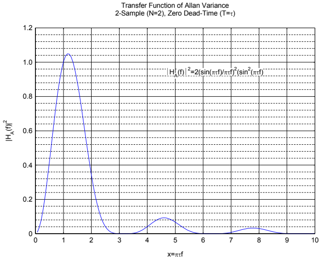
Allan Variance
