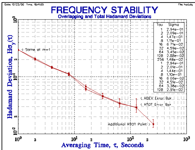
Overlapping & Total Hadamard Deviations
