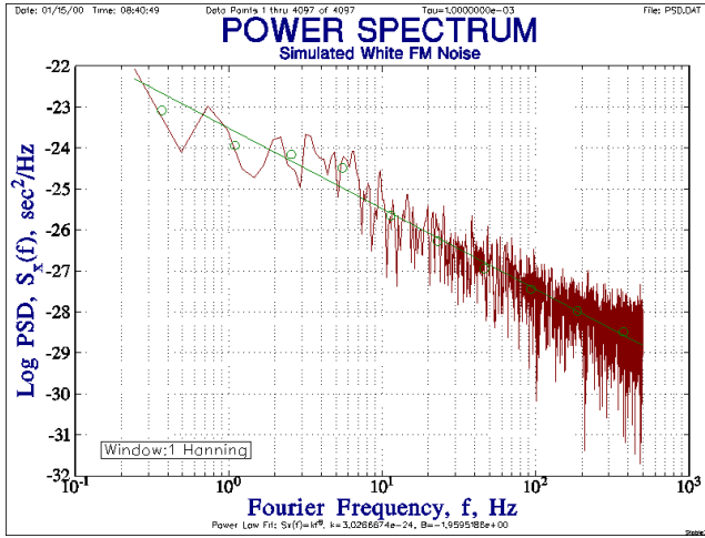
Figure 7.2e S_x(f) Power Spectral Density
