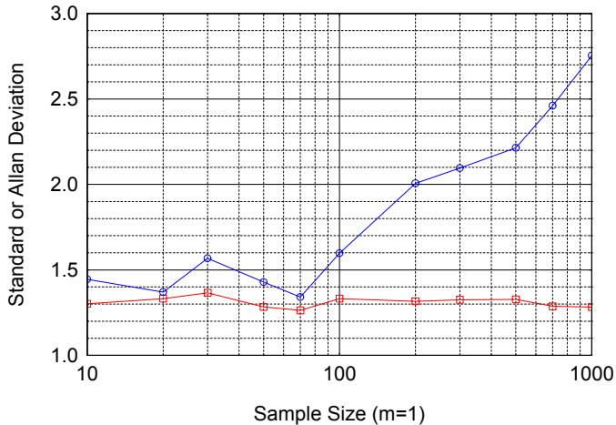
Convergence of Standard &amp; Allan Deviation for F FM Noise
