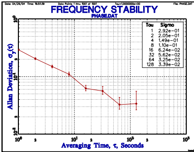
Original Allan
