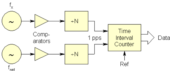
Figure 9.1 Block Diagram of a Time Interval Counter Measuring System
