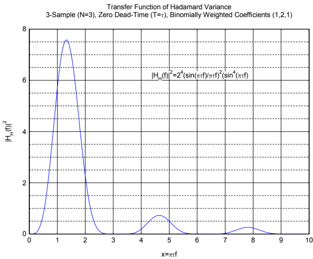
Hadamard Variance
