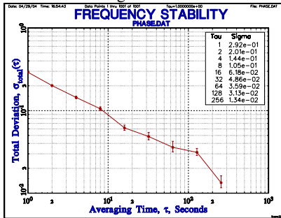
Total
