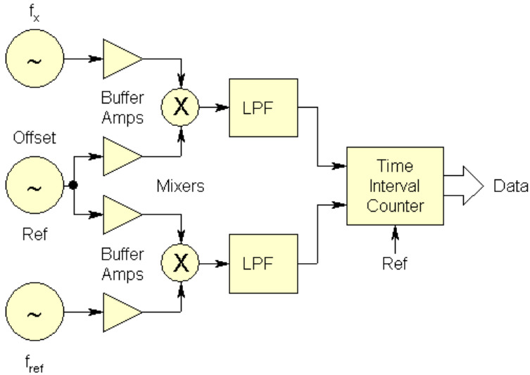
Figure 9.3 Block Diagram of a Dual Mixer Time Difference Measuring System
