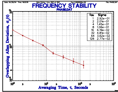
Overlapping Allan
