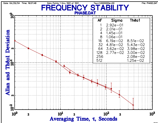
Overlapping & Théo1
