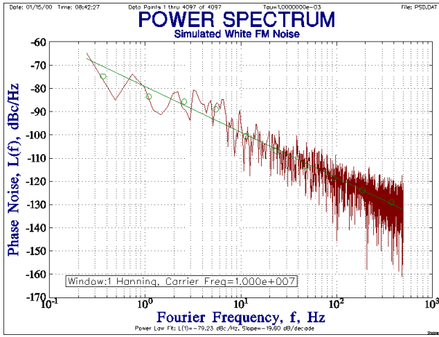
Figure 7.2c \mathbf{L}(f) Power Spectral Density
