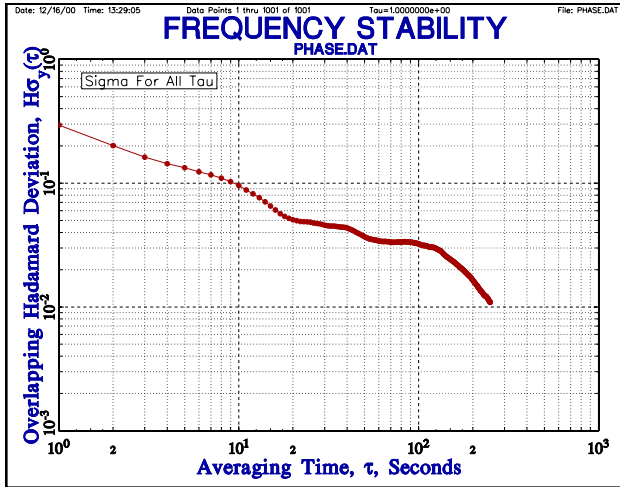
Overlapping Hadamard Deviation
