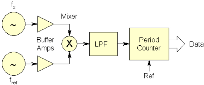
Figure 9.2 Block Diagram of a Heterodyne Measuring System
