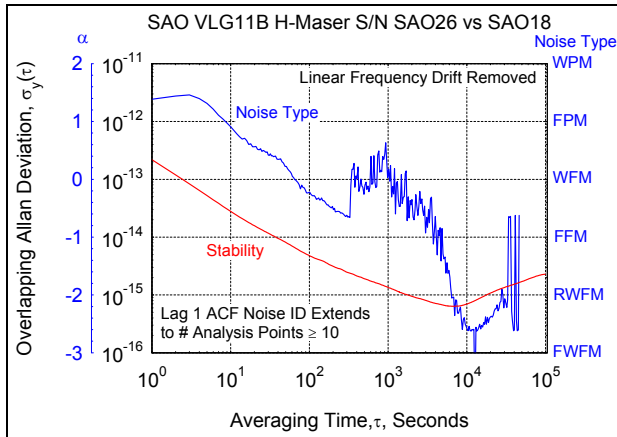
Frequency Stability and Noise Analysis of Two Hydrogen Masers
