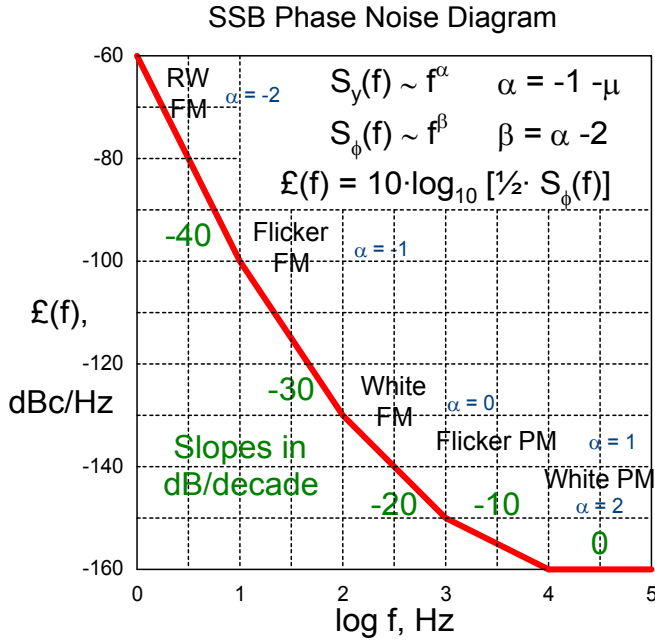
Figure 6.3 SSB Phase Noise Plot
