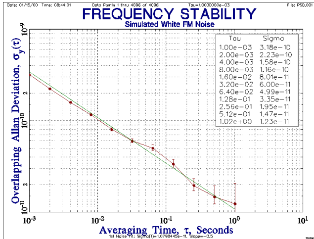
Figure 7.2b Overlapping Allan Deviation
