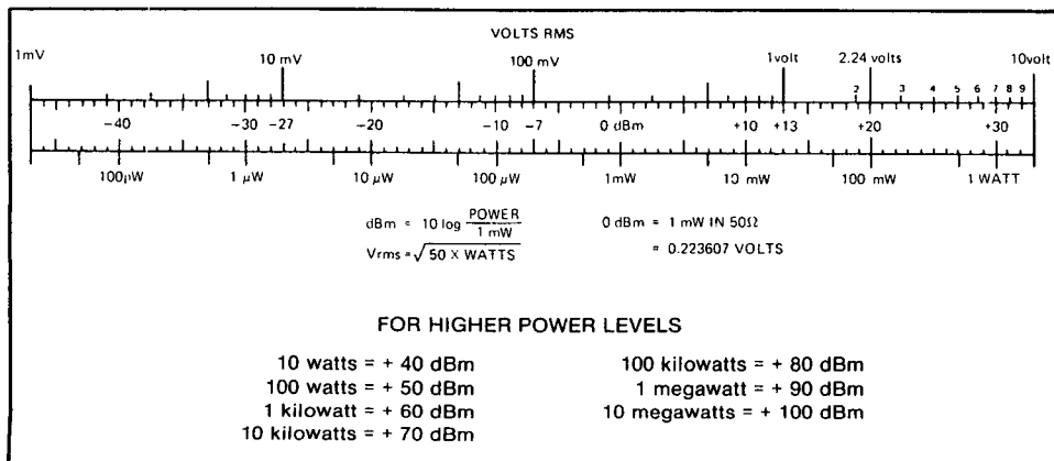
FIGURE IV-2 Nomograph relating dBm, watts and volts for a 50 ohm system.
