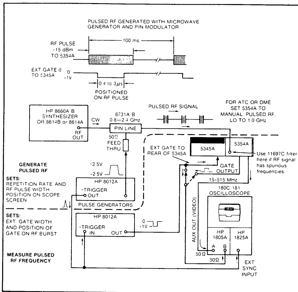
FIGURE IV-4 Frequency averaging of pulsed RF signal using EXT GATE for increased resolution and accuracy.
