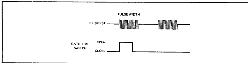
FIGURE IV-6 For INT ARM, GATE TIME must be less than pulse width.
