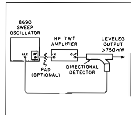
Figure 5. The E15-8690A system generates high-level (750 mW), flat output power. The pad between the sweep oscillator and the TWT amplifier is used to keep the signal level into the amplifier below that which would saturate the TWT.
