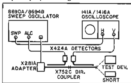
Figure 3. Typical Waveguide Reflectometer.
