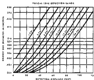
Typical leak detection ranges of HP ultrasonic translators. Curves give typical leak detection distances for orifice type leads versus pressure and orifice size.
