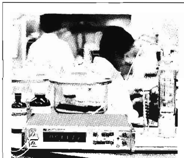
2801A Quartz Thermometer being used with a differential ebulliometer to measure boiling point elevation of a solution, from which the solute molecular weight is derived.
