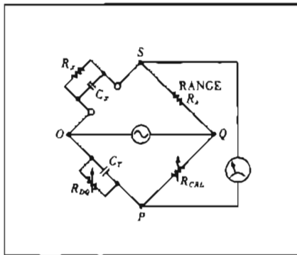
Figure 1. Generalized ac bridge configuration. OQ is bridge driving voltage. OS is fixed by value of unknown component and setting of RANGE switch. OP is determined by R_{CR1} and R_{D0} controls and C_T . When balanced, voltage across PS is zero.
