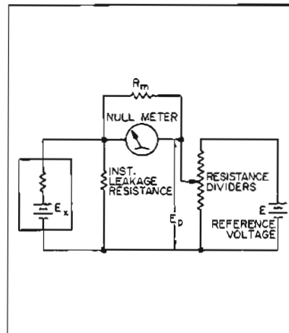
Figure 5. Classic differential voltage measurement.
