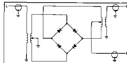
Figure 2. Ring Modulator
