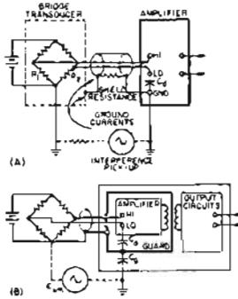
Figure 5. Guard reduces capacitance between signal leads and ground.
