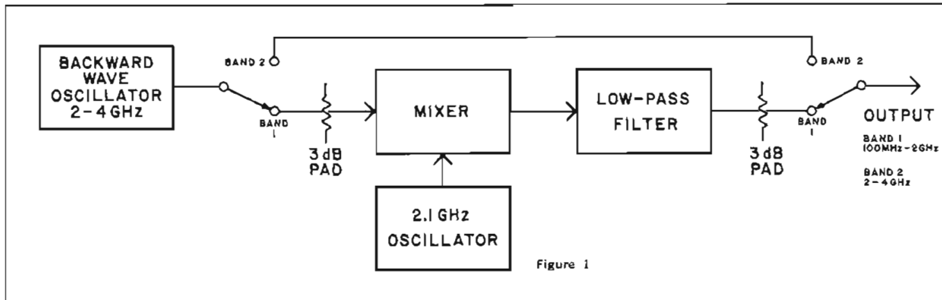
Model 8701A RF Unit Block Diagram
