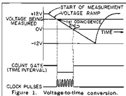
Figure 1. Voltage-to-time conversion.
