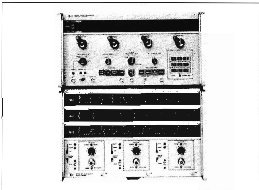
Figure 2. Models 8706A Control Unit and 8707A RF Unit Holder with 8690A Sweep Oscillator.
