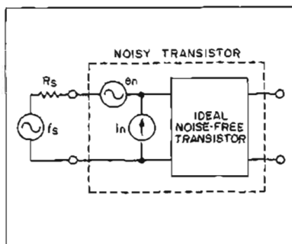
Figure 1. Transistor Noise Model
