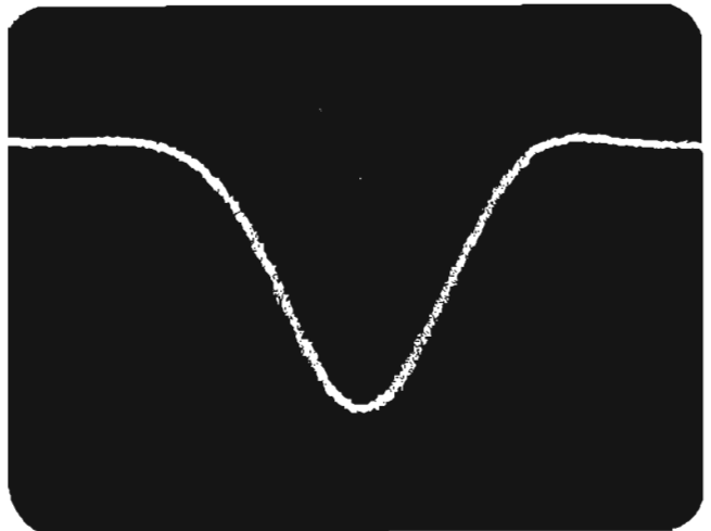
CRT display using Model 1815A/1817A/1106A TDR system slows the reflection from HP Model 8748 Susceptance Standard set at 1 pF equivalent capacitive discontinuity. Scale: 20 ps/div horizontal, 0.1 p/div vertical.
