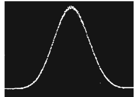
Probability density function of pseudo-random Gaussian noise (same sequence as at left) displayed on Model 5400A Multi-channel Analyzer.
