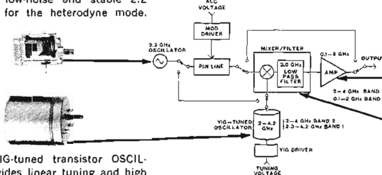
8699B Block Diagram
