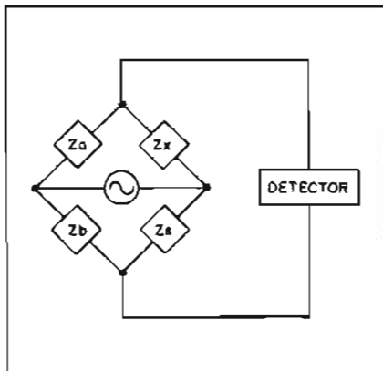
Figure 1. Generalized Bridge Circuit
