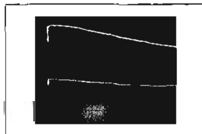
Figure 11. Transistor Current Gain—Current gain ( B ) may be measured using the current probes. This is a power transistor whose gain is 33 dB at 1 MHz (sweep is 1 to 10 MHz to 1 MHz per division). Amplitude is 10 dB/division, phase 100°/division, showing 16 dB gain at 10 MHz and a flat phase response (about 45° from 1 to 10 MHz). Center of graticule is 0 dB and 0^\circ phase reference.
