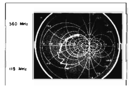
Figure 22. Swept-frequency display of impedance of a tunnel diode when it is biased in the negative impedance region.
