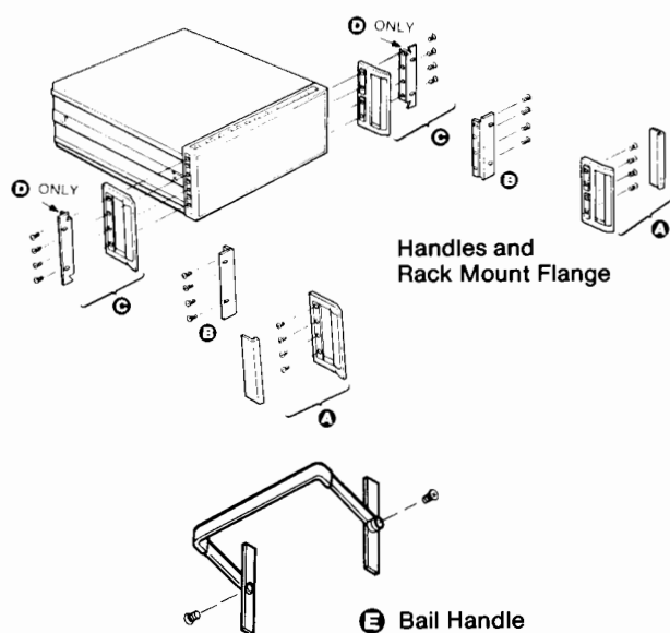
Bail Handle
