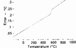
100 \Omega Platinum RTD \alpha = .00385 (90 day specifications)
