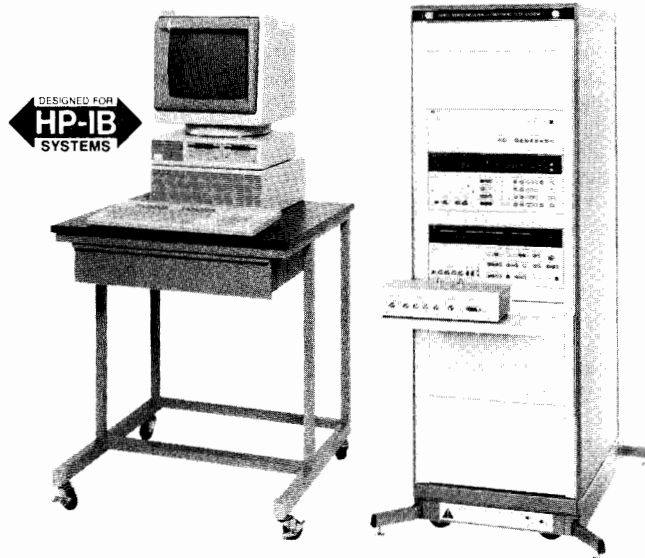
HP 4061A
