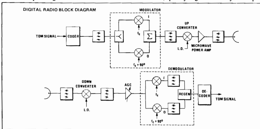
Digital Radio Block diagram
