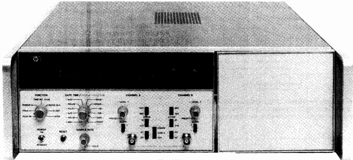
HP 5345A
