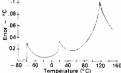
2.2 k \Omega Thermistor (90 day specifications)
