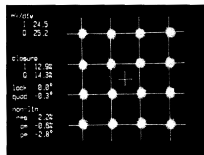
Constellation Pattern from the HP 3709B showing measurements (16 QAM radio)
