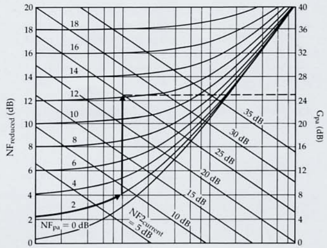
Figure 5.3 Graph to calculate preamp noise figure and gain. (Procedure for use is given in text.) Example shown: To reduce NF2_{\text{current}} (25 dB) to NF2_{\text{reduced}} (4 dB), a 2 dB noise figure, 25 dB gain preamplifier is needed.
