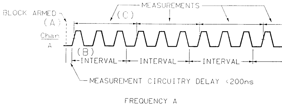
Figure 5-18. INTERVAL SAMPLING Timing Diagram
