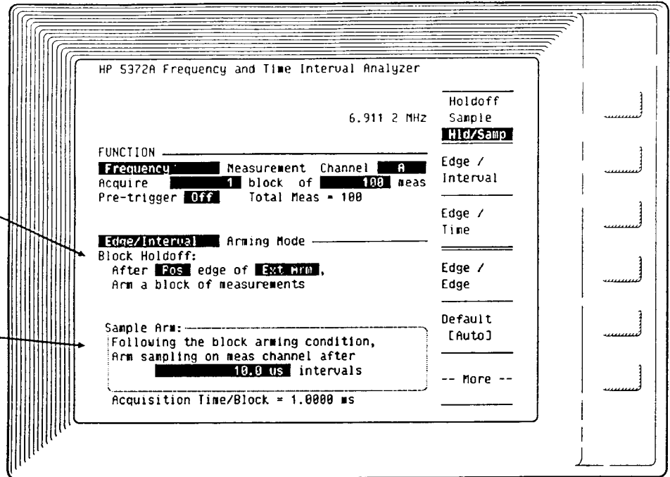
Figure 2-4. Arming Mode Text and Explanation
