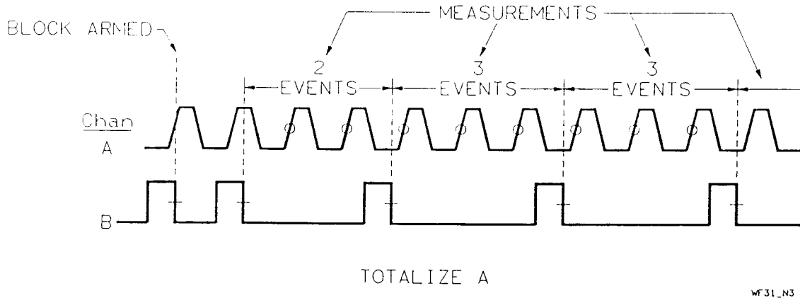
Figure 3-4. Totalize | Edge/Edge
