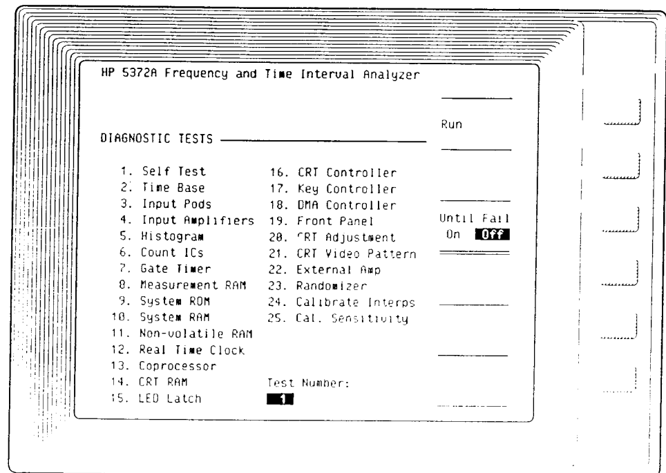
Figure 13-1. Test Menu Screen
