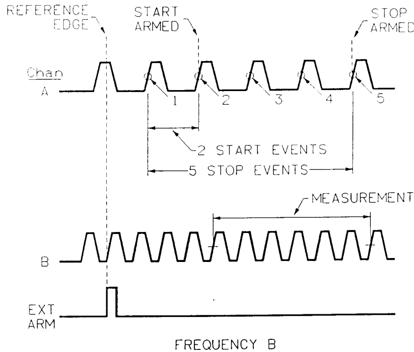
Figure 2-22. Frequency | Event/Event
