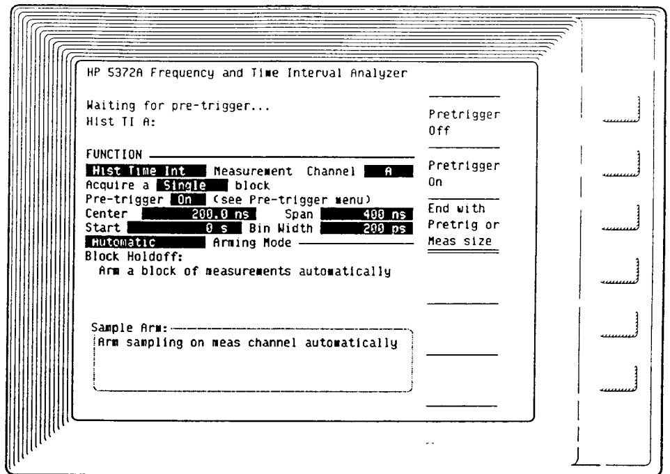
Figure 4-9. Setup 4: Single Block — Measurements End on Pre-trigger
