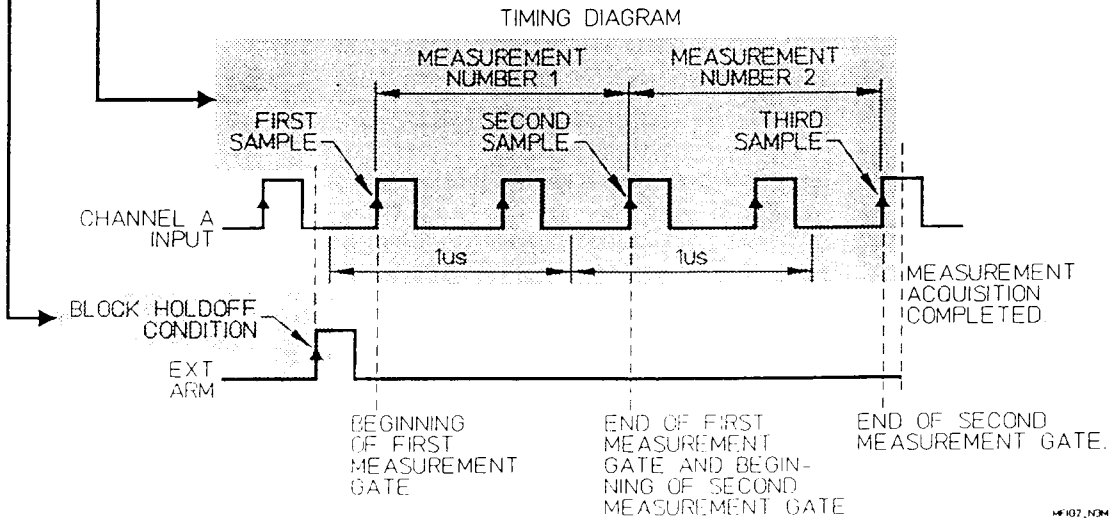
Figure 5-2. Group of Measurements
