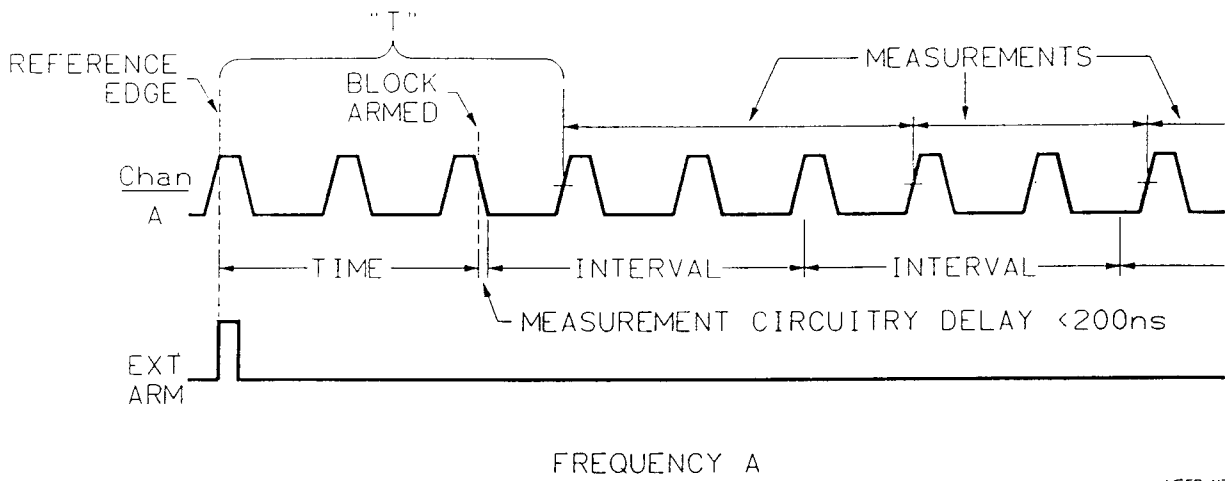
Figure 2-19. Frequency | Time/Interval
