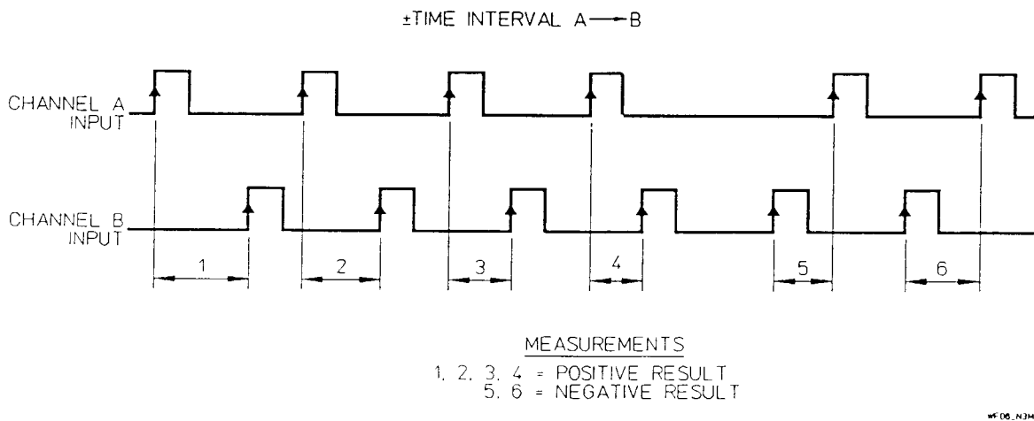
Figure 1-7. \pm Time Interval on Two Channels
