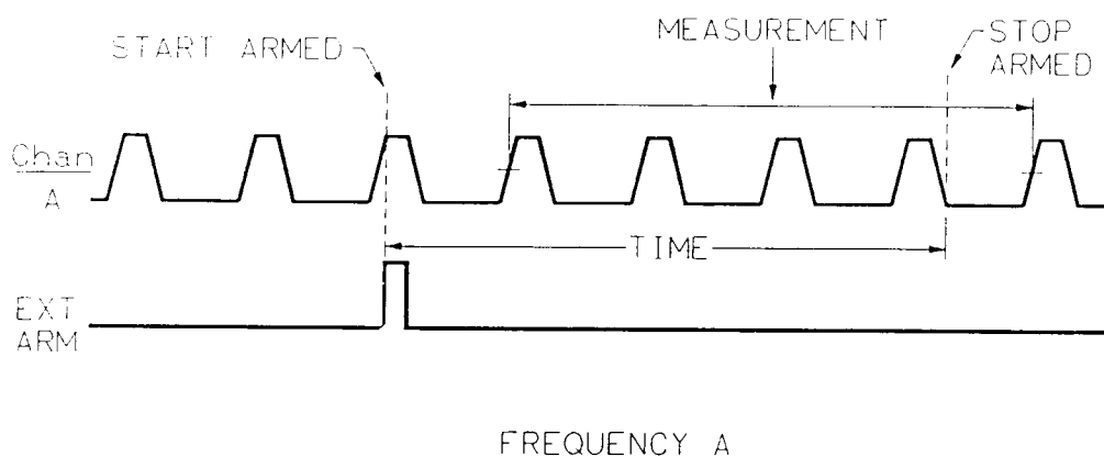
Figure 2-15. Frequency | Edge/Time
