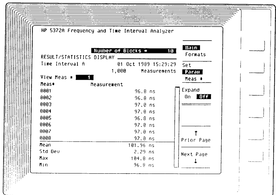
Figure 15-3. Result/Statistics Display
