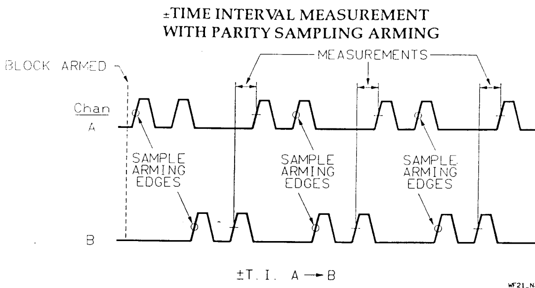
Figure 1-36. ±Time Interval | Parity Sampling
