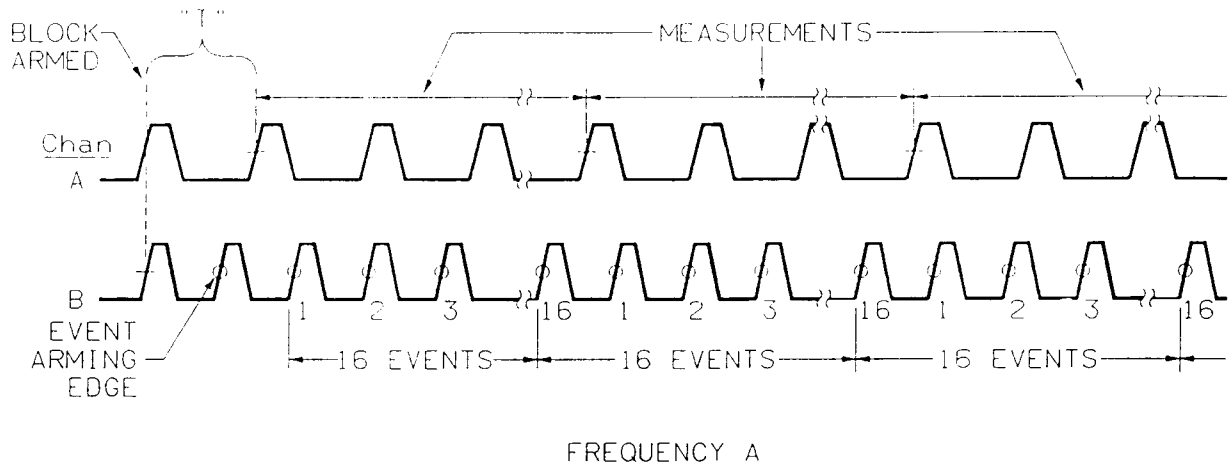
Figure 2-17. Frequency | Edge/Cycle
