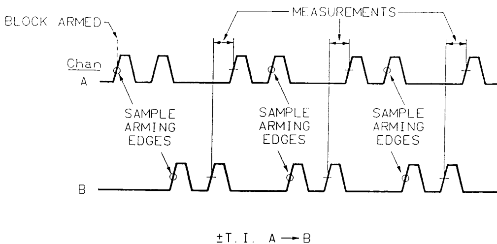
Figure 1-42. ± Time Interval | Edge/Parity
