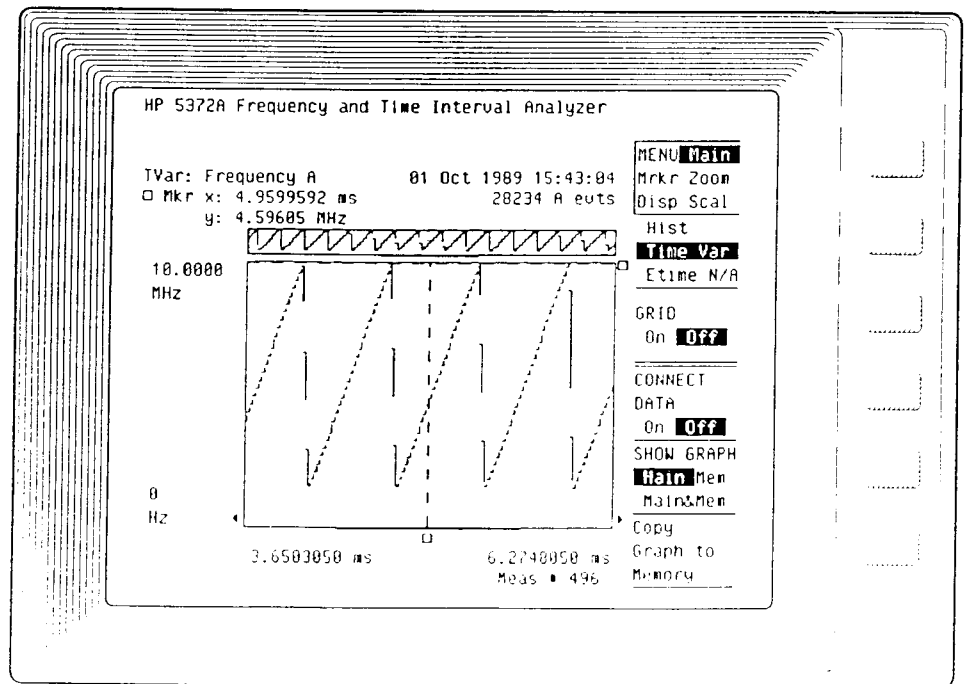
Figure 16-1. Main Menu for a Time Variation Graph
