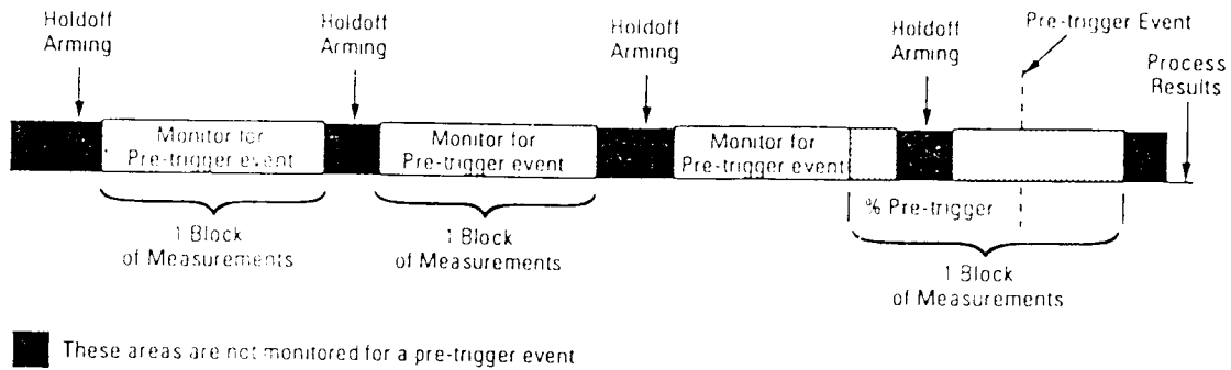
Figure 10-3. Pre-trigger Operation on Multiple Blocks of Measurements
