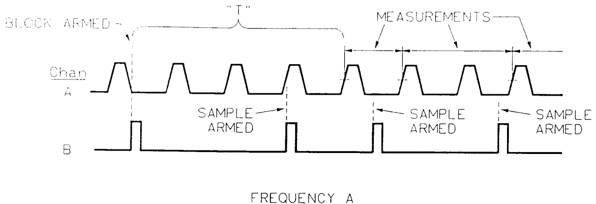
Figure 2-16. Frequency | Edge/Edge
