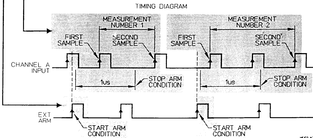
Figure 5-3. Separate Measurements
