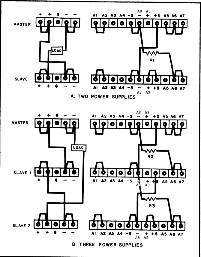
Figure 3-10. Auto-Series, Two and Three Units
