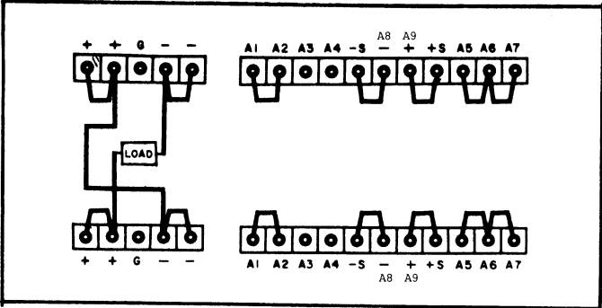
Figure 3-9. Normal Series Connections
