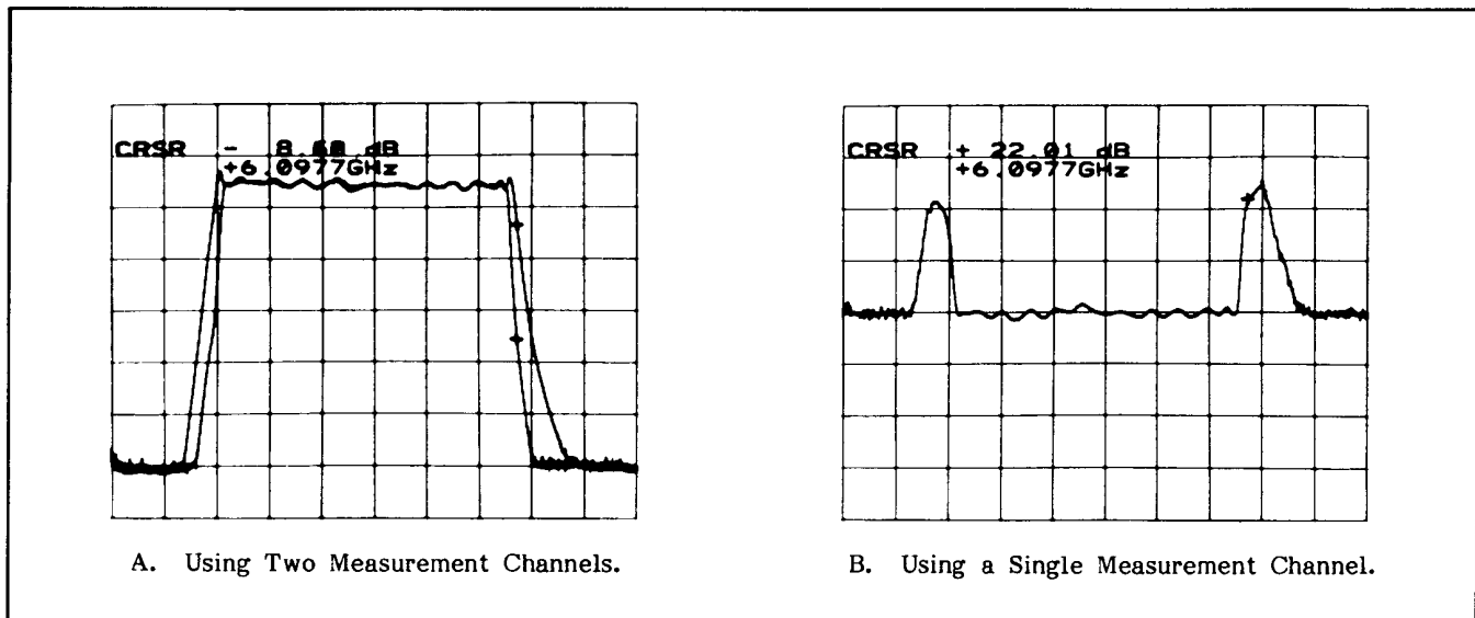
Figure 15. Matching Devices
