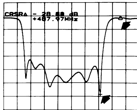
D. After CURSOR MAX, CURSOR Δ ON, CURSOR MIN.
