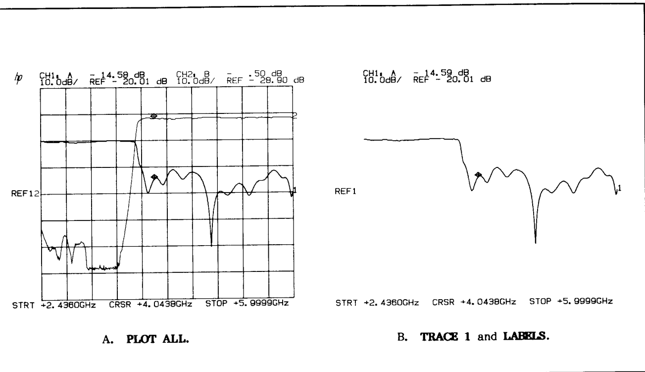
Figure 13. Examples of Plotter Output
