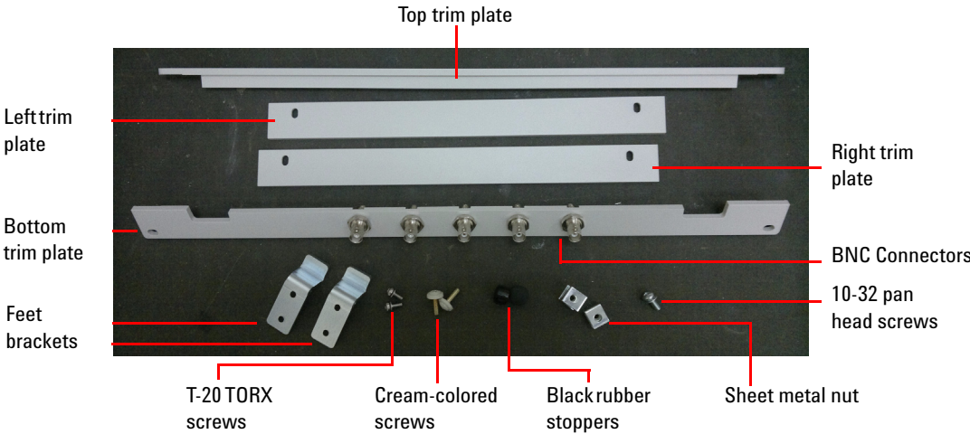
Figure 1-16 Trim plates, foot brackets, T-20 TORX screws, cream-colored screws, black rubber stoppers, sheet metal nut, and 10-32 pan head screws
