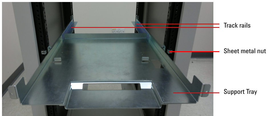
Figure 1-15 Track rails, sheet metal nut, and support tray
