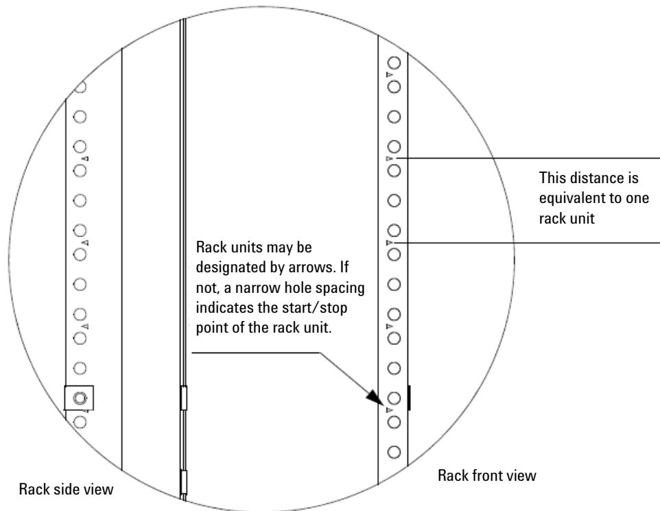
Figure 1-17 Rack unit
