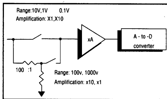
Figure 2. The DC input path to the analog-to-digital converter is either through an amplifier only or through an additional resistive attenuator, depending on the range used.
