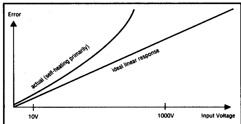
Figure 3. On the 1000 V range, nonlinear self-heating errors of the 100:1 resistive attenuator are noticeable.
