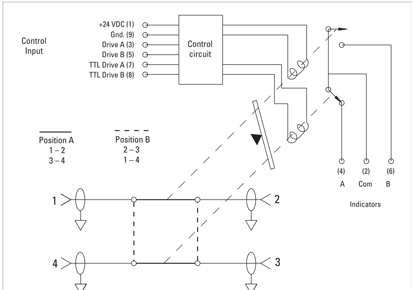
Figure 1. Keysight 87222C/D/E schematic
