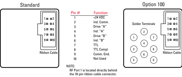
Figure 8. Drive connections
