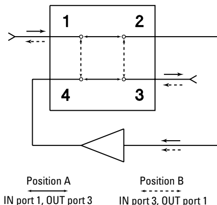
Figure 4. Signal reversal
