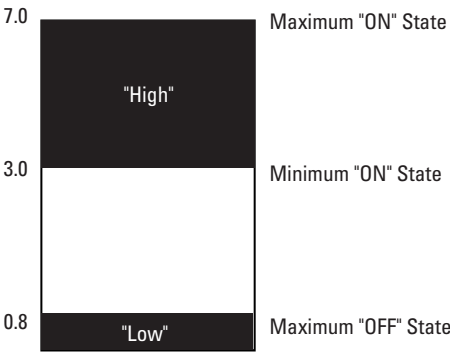
Figure 9. TTL control voltage states
