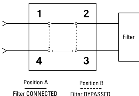
Figure 3. Drop-out switch
