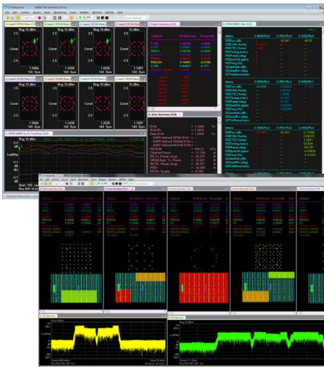
LTE-Advanced 8x8 MIMO analysis showing per layer error traces and tables as well as frequency response trace color-coded for each layer.
