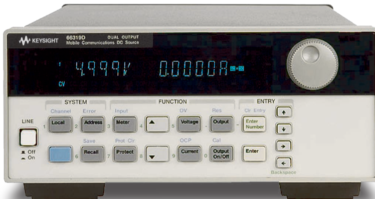
66319D Dual Mobile Comm DC Source with Battery Emulation
