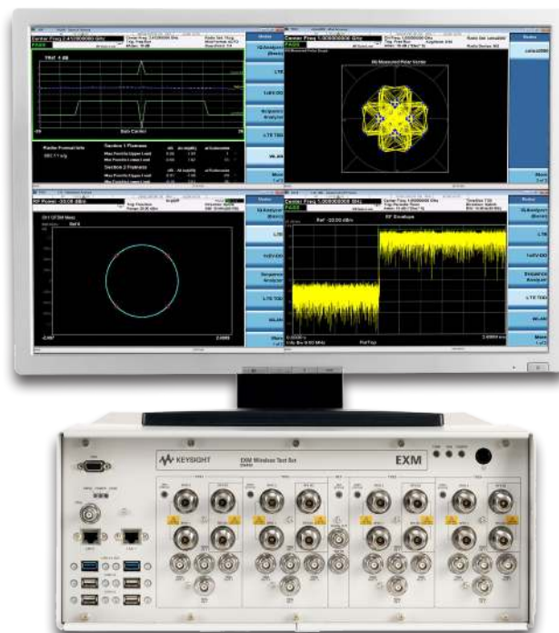
Use the EXM with four TRX channels to parallel test wireless devices. WLAN, cdma2000, LTE FDD and LTE TDD shown.
