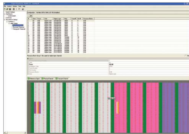
Flexible resource mapping with scalable system bandwidth is available with Keysight's Signal Studio Software.
