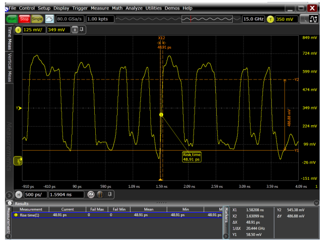
Figure 6. InfiniiScan measurement finder identifies a rise-time slower than 50 ps in order to locate ISI issues that are occurring on a single-bit pulse
