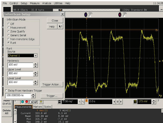
Figure 11. InfiniiScan's runt finder can be used to isolate runt pulses that occur in a signal.
