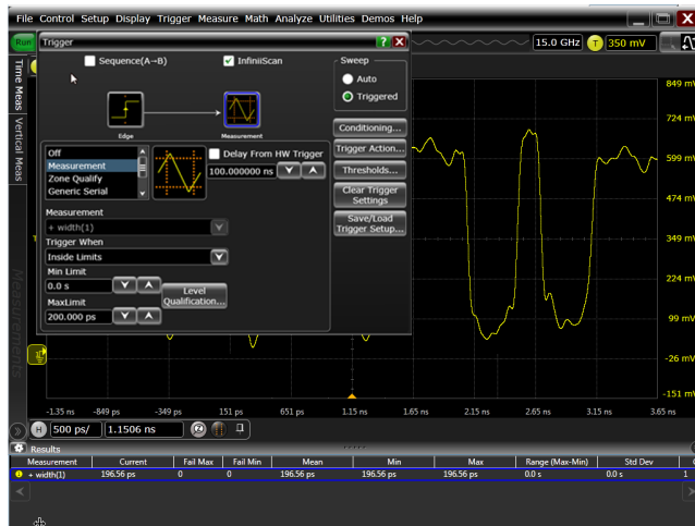
Figure 5. InfiniiScan measurement finder identifies a glitch that occurs under 200 ps
