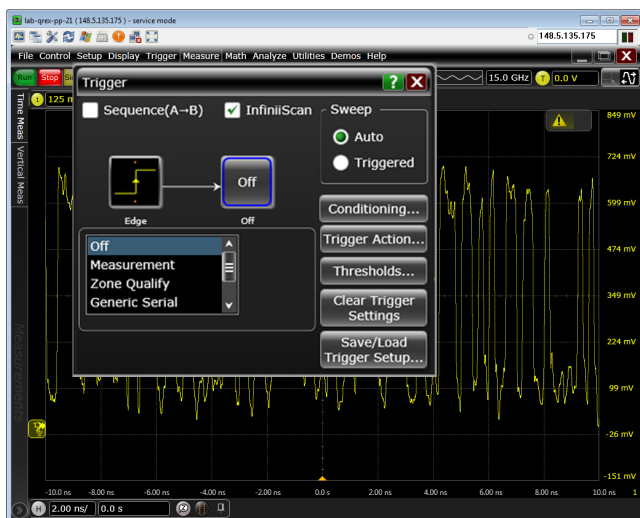
Figure 1. InfiniiScan menu is conveniently located by the trigger menu
