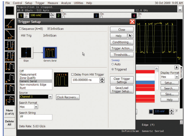
Figure 10. InfiniiScan's generic serial finder is used to isolate a specific portion of a high-speed serial data stream.
