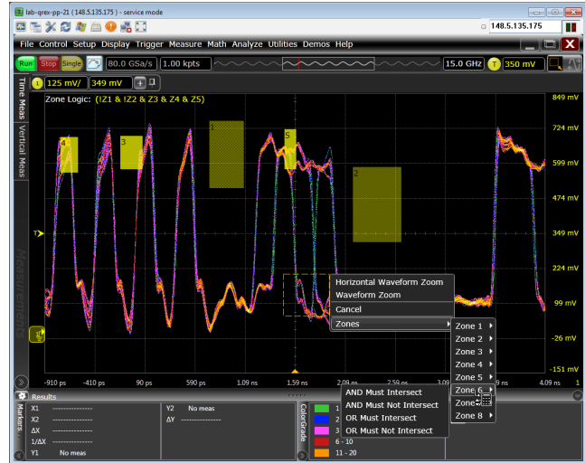
Figure 8. Notice how zone qualify is able to easily isolate the exact signal you need. This is very useful for many applications, including separating reads and writes for memory signals.
