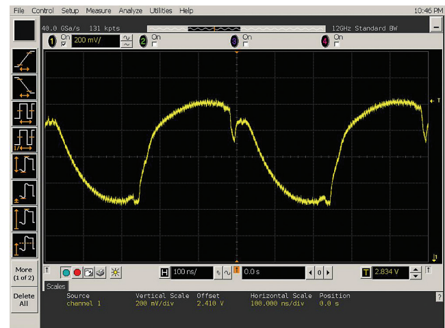
Figure 12. InfiniiScan's non-monotonic edge finder isolates a signal anomaly caused by a poor termination.
