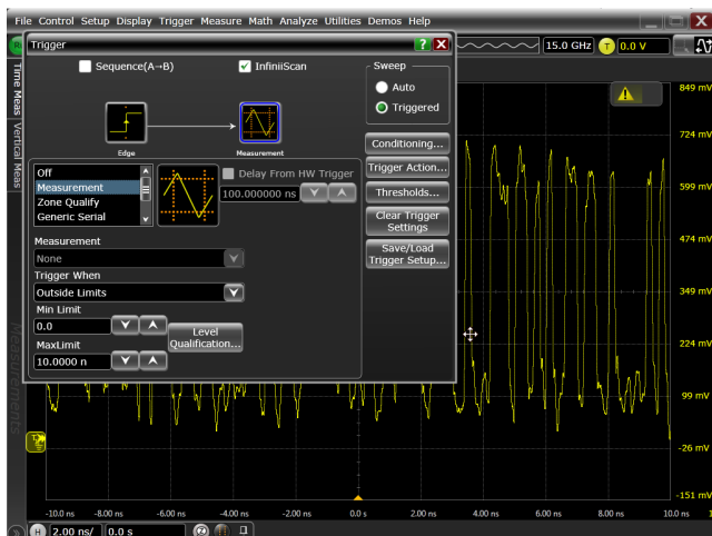
Figure 3. Limit test search allows you to quickly see how many failures you have and then step through the failures one by one
