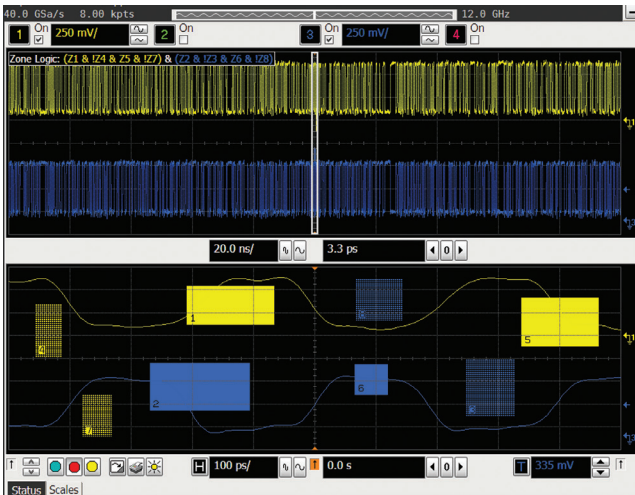
Figure 7. The InfiniiScan zone qualify finder is used to isolate single-bit pulses. Only the waveforms that pass the must-not-intersect (upper left) and must-intersect (lower right) graphical zones are displayed.
