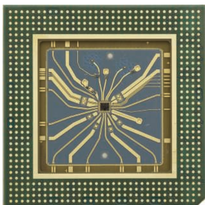
Keysight's uses Indium Phosphide to produce a sub 12 ps edge perfect for characterizing cable and probe frequency response
