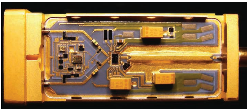
The InfiniiMax III probing system uses the same InP technology that enables high bandwidth and low noise oscilloscope measurements.
