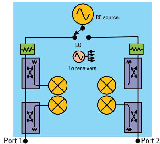
Figure 10: N9923A with option 122
