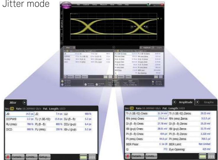
Precision jitter, amplitude, and frequency analysis capability
