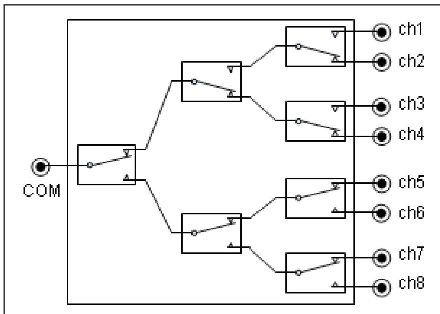
Figure 7. M9148A and M9152A 1x8 RF switch multiplexers
