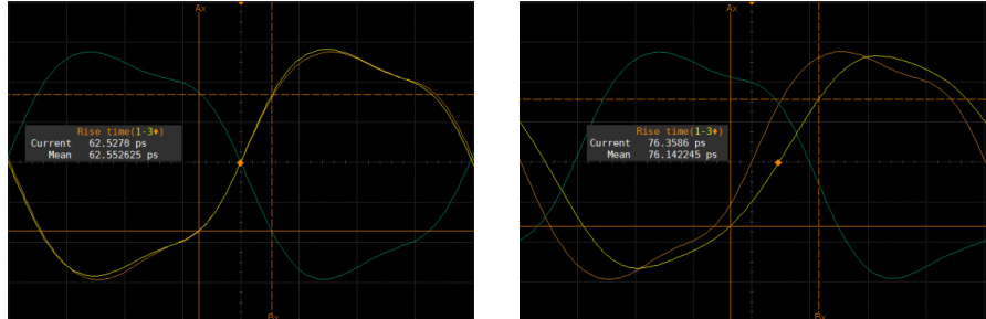
Figure 7. Rise time degradation due to 50 ps of skew. The differential signal is shown in the yellow trace
