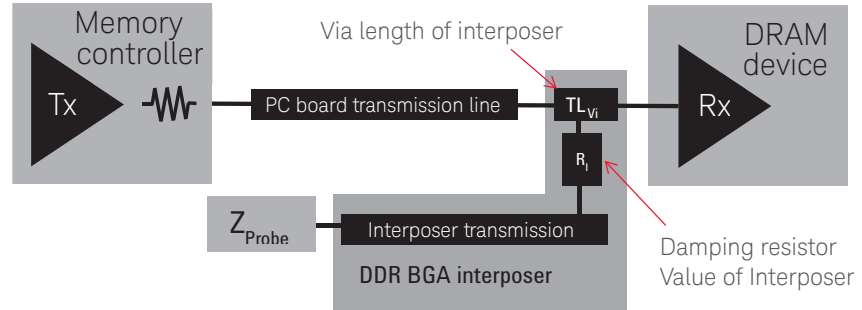
Figure 34. Circuit diagram of DDR interposer
