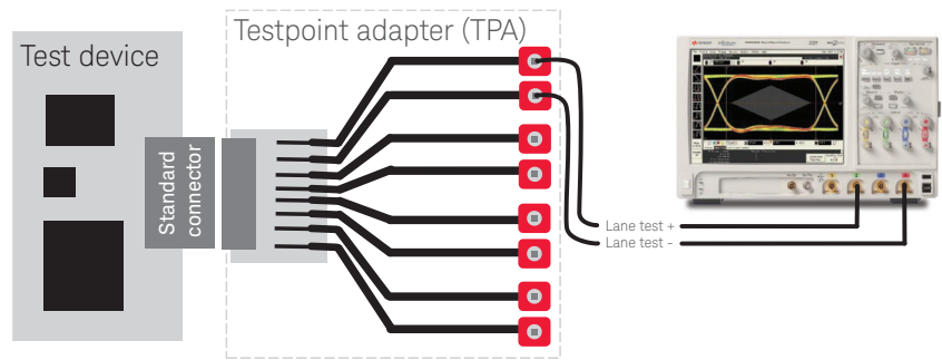
Figure 3. Test device has a digital standard connector, not an RF coaxial launch
