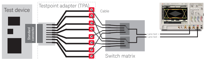
Figure 5. Case 2 with switching network. All lanes are connected to this switch matrix
