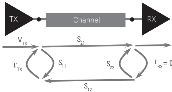
Figure 9. Flow graph analysis of system
