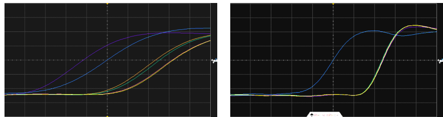
Figure 21. Comparisons of skew before and after compensation with PrecisionProbe ( \pm 2 ps)
