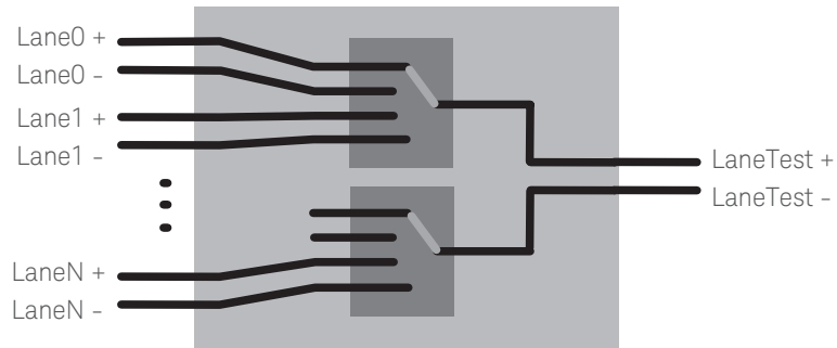
Figure 1. Two multi-port microwave switches can be used to switch high speed differential lanes
