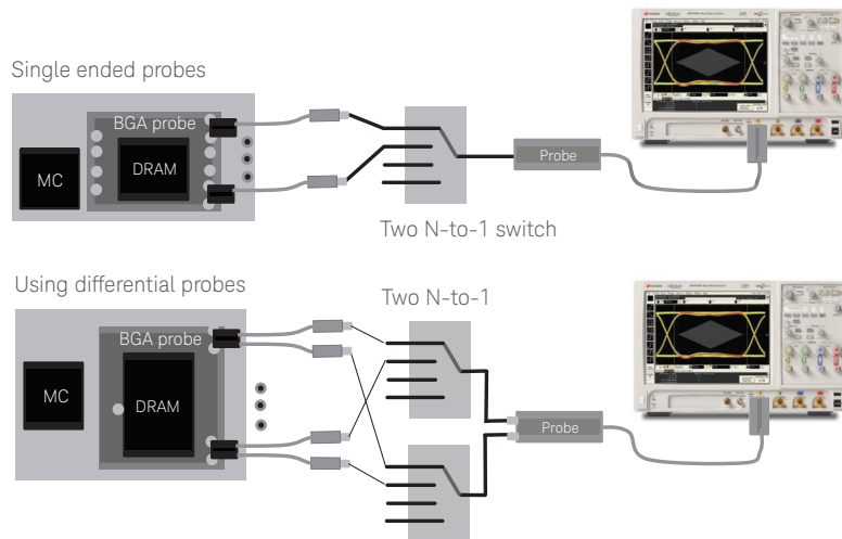
Figure 35. DDR switching
