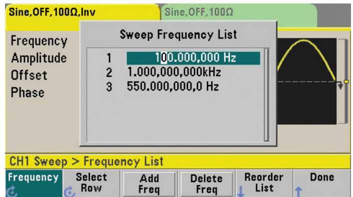
Figure 2. Trueform waveform generator frequency list menu.
