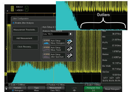
Figure 3: Jitter analysis using a TIE histogram plot.
