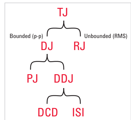
Figure 9: Jitter components.
