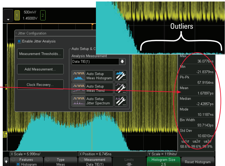
Figure 3: Jitter analysis using a TIE histogram plot.
