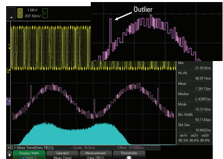
Figure 4: TIE jitter trend waveform shows sinusoidal modulation along with extreme timing errors.
