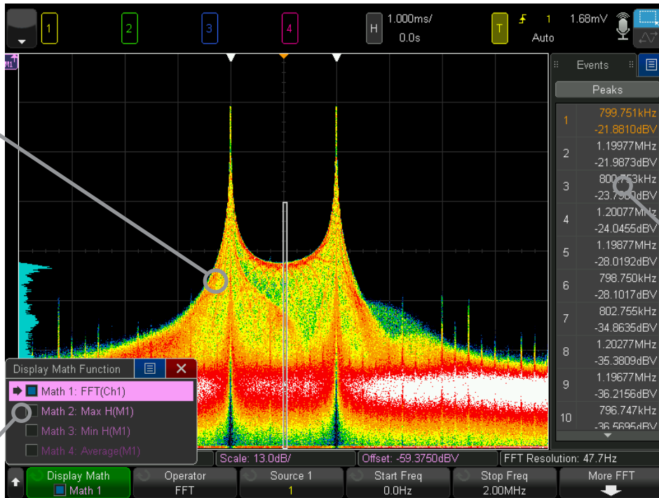
Figure 37. Enhanced color FFT.
