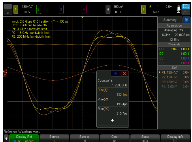
Figure 51. Reference waveforms.
