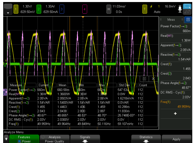
Figure 43. Power quality analysis screenshot.
