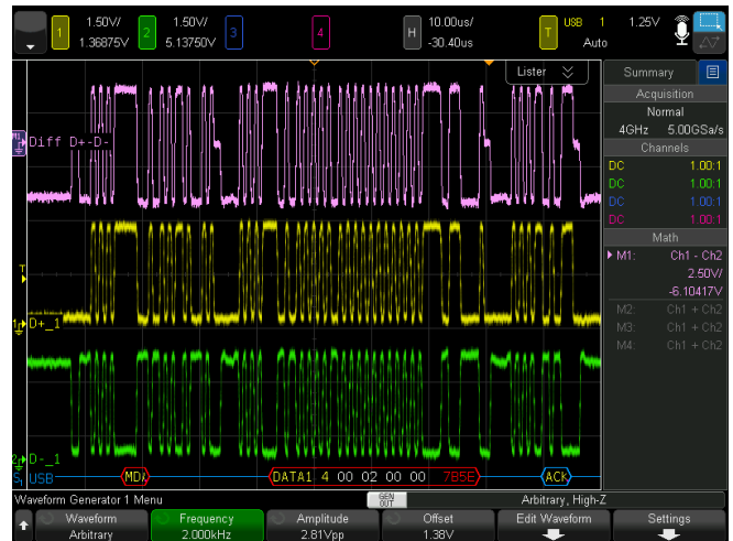
Figure 29. Dual-channel generator generating a differential signal.
