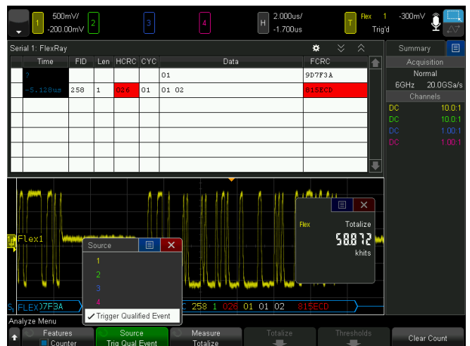
Figure 34. Totalizing the number of CAN errors.
