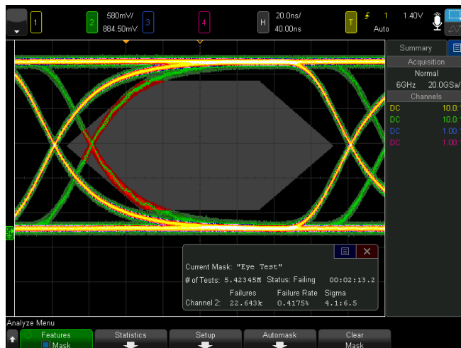
Figure 41. Mask testing of serial data.
