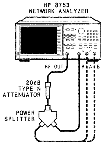
Figure 1. Operator's Check Equipment Setup.
