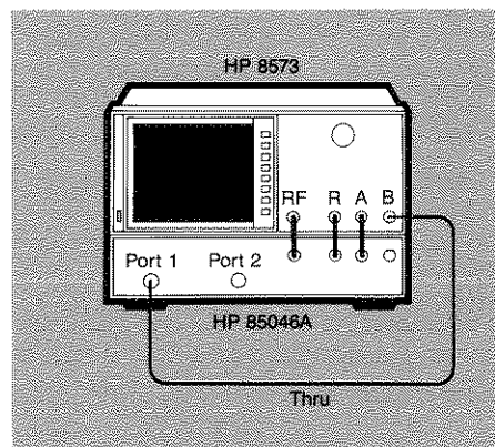
Figure 13. Setup for calibration to input B.
