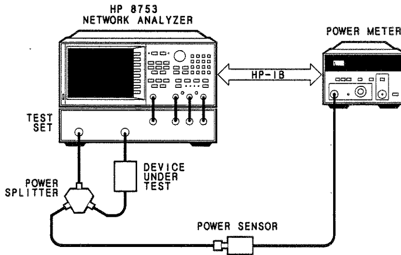
Figure 5-19. Typical Test Setup for Continuous Correction
