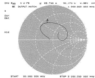
Figure 11. Complex impedance measurement.
