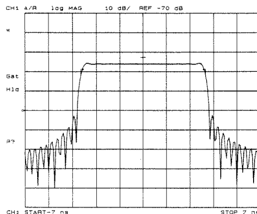
Figure 8-16. Gate Shape
