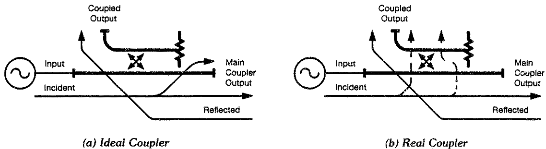
Figure 5-1. Directivity
