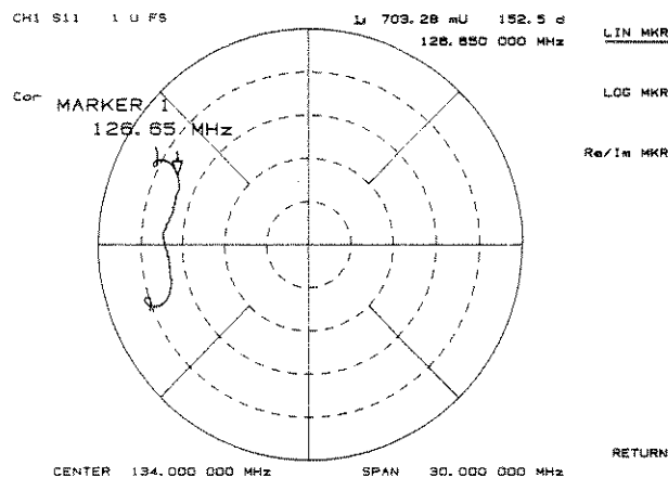
Figure 4-14. Polar Format
