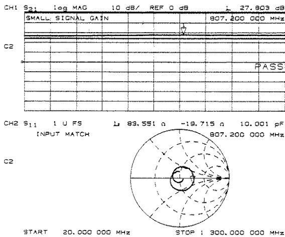
Figure 1. Display of amplifier gain and input match
