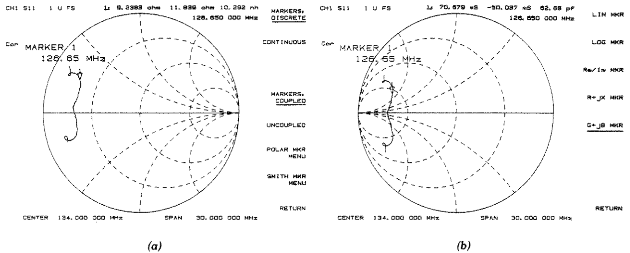
Figure 4-13. Standard and Inverse Smith Chart Formats
