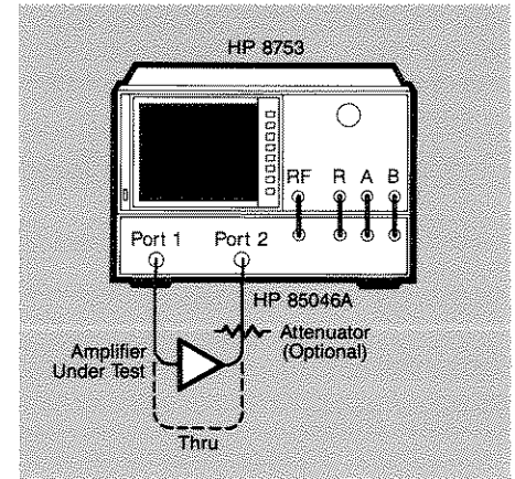
Figure 3. Basic setup for amplifier measurements using the HP 8753 with a S-parameter test set.
