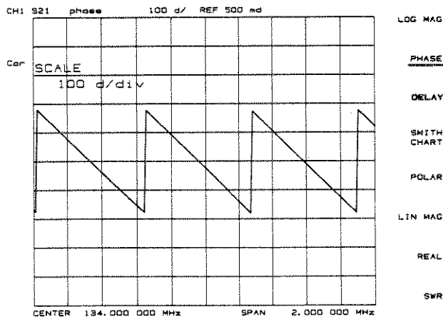
Figure 4-11. Phase Format
