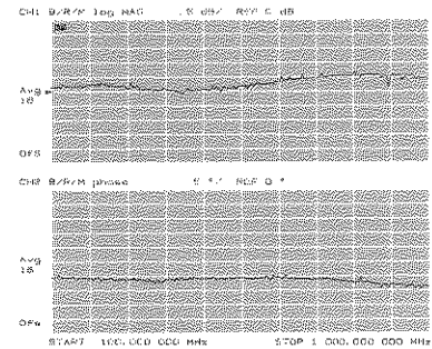
Figure 15. Plot of amplitude and phase tracking between two mixers.
