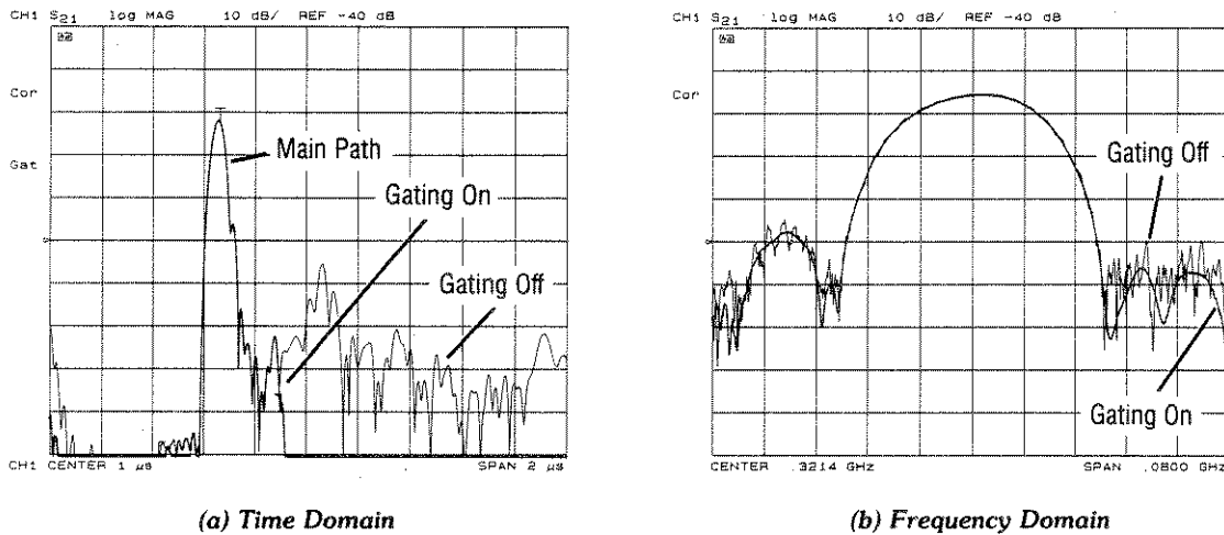
Figure 8-15. SAW Filter Transmission Measurement with Gating
