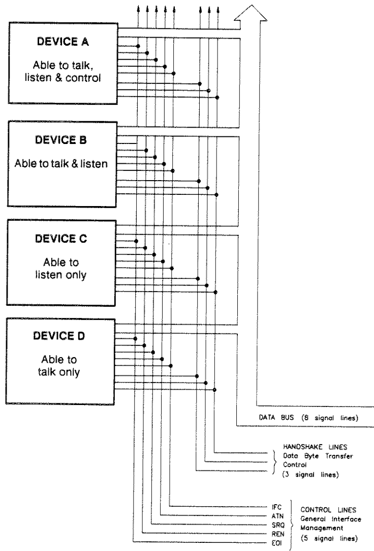
Figure 11-1. HP-IB Structure
