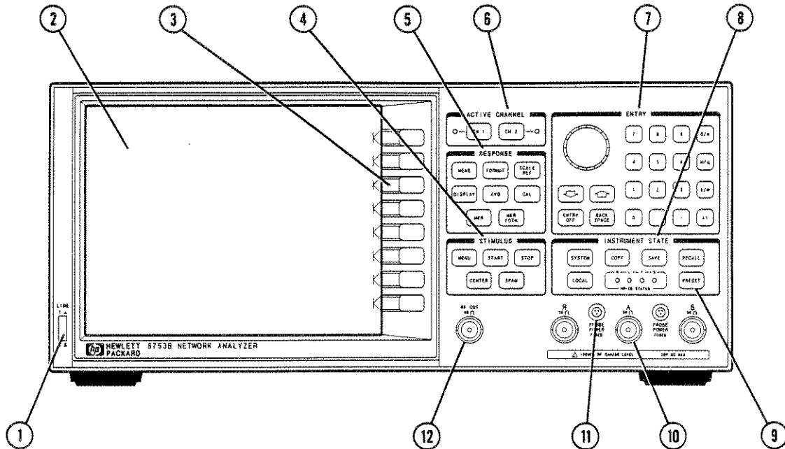
Figure 2-1. HP 8753B Front Panel
