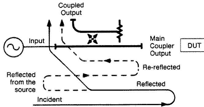
Figure 5-2. Source Match
