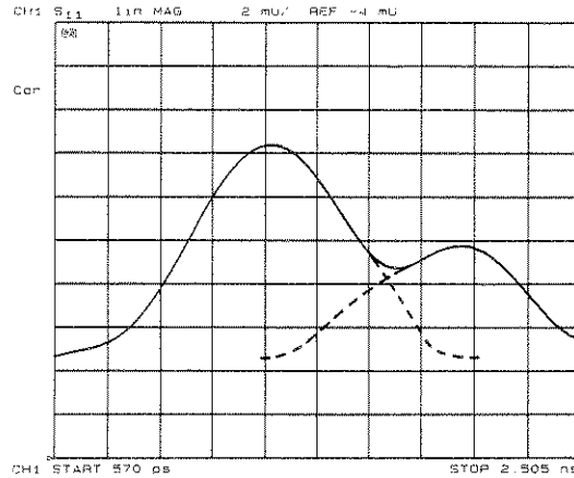
Figure 8-13. Response Resolution
