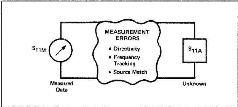
Figure 5-32. Sources of Error in a Reflection Measurement
