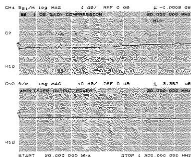
Figure 12. Swept frequency gain compression measurement.
