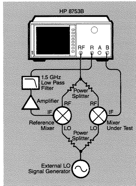
Figure 9. Block diagram for a conversion loss measurement greater than 35 dB.
