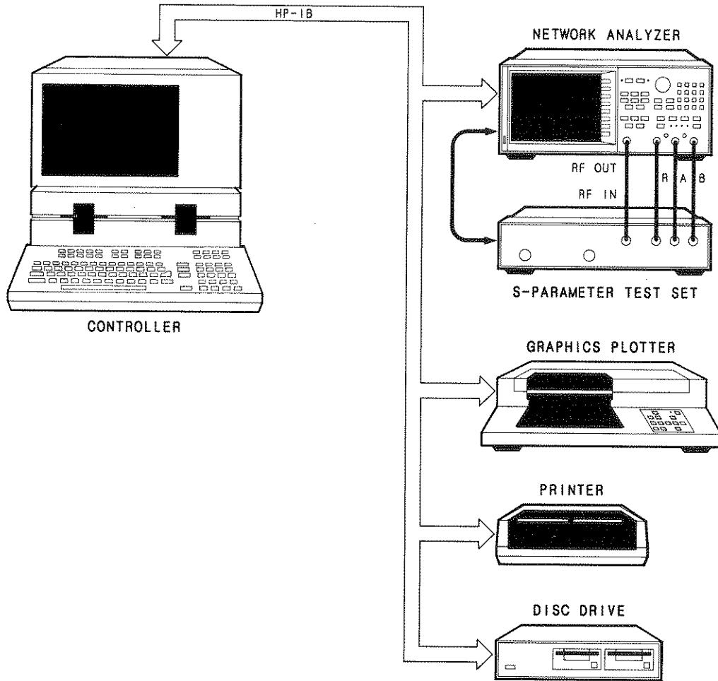
Figure 4. HP-IB Connections in a Typical Setup
