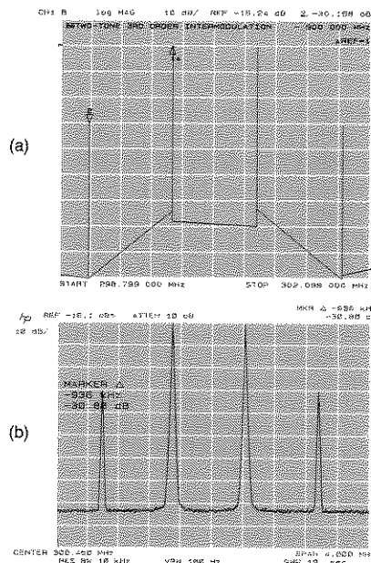
Figure 18. Two-tone IMD measurement (a) using the HP 8753B and (b) using a Spectrum Analyzer.
