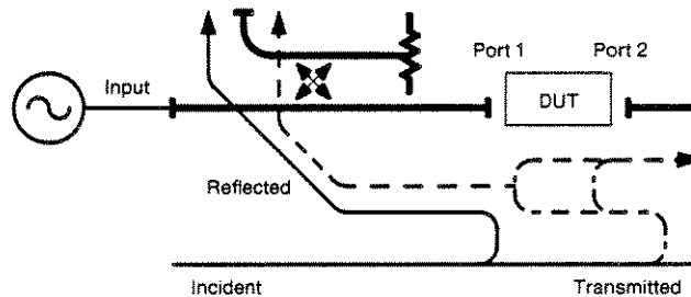
Figure 5-3. Load Match
