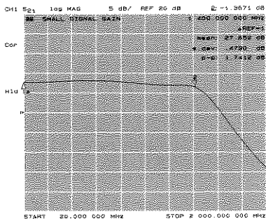
Figure 4. Small signal gain measurement.
