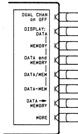
Figure 4-24. Display Menu
