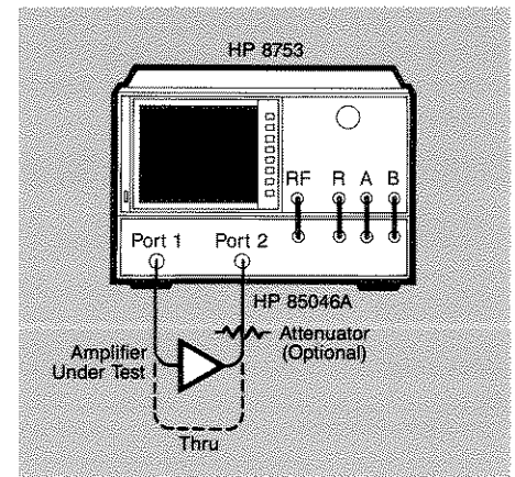
Figure 3. Basic setup for amplifier measurements using the HP 8753 with a S-parameter test set.
