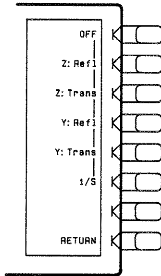
Figure 4-8. Conversion Menu
