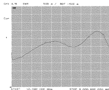
Figure 21. Plot of a mixer's RF port SWR.
