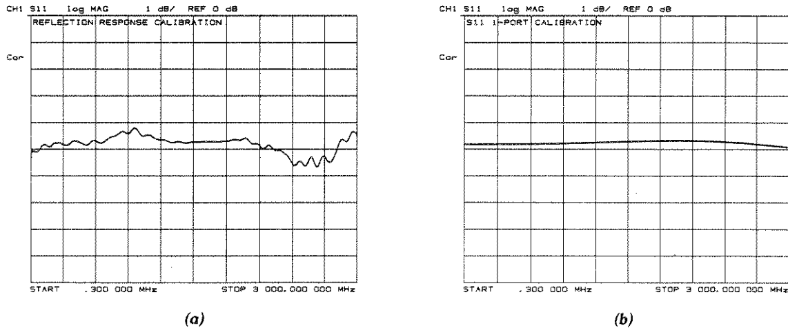
Figure 5-4. Response vs. S_{11} 1-Port Calibration on Log Magnitude Format
