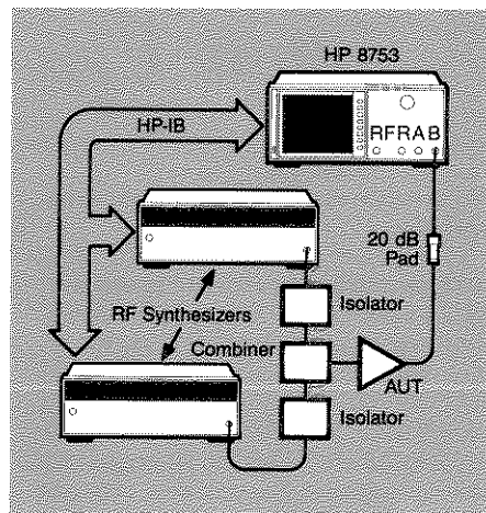
Figure 19. Two-tone third order intermodulation measurement setup.
