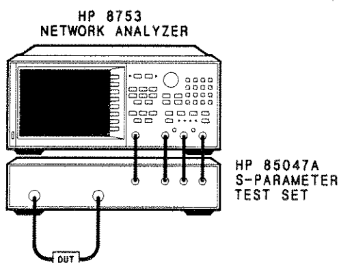
Figure 14-7. Typical Harmonic Mode Test Setup
