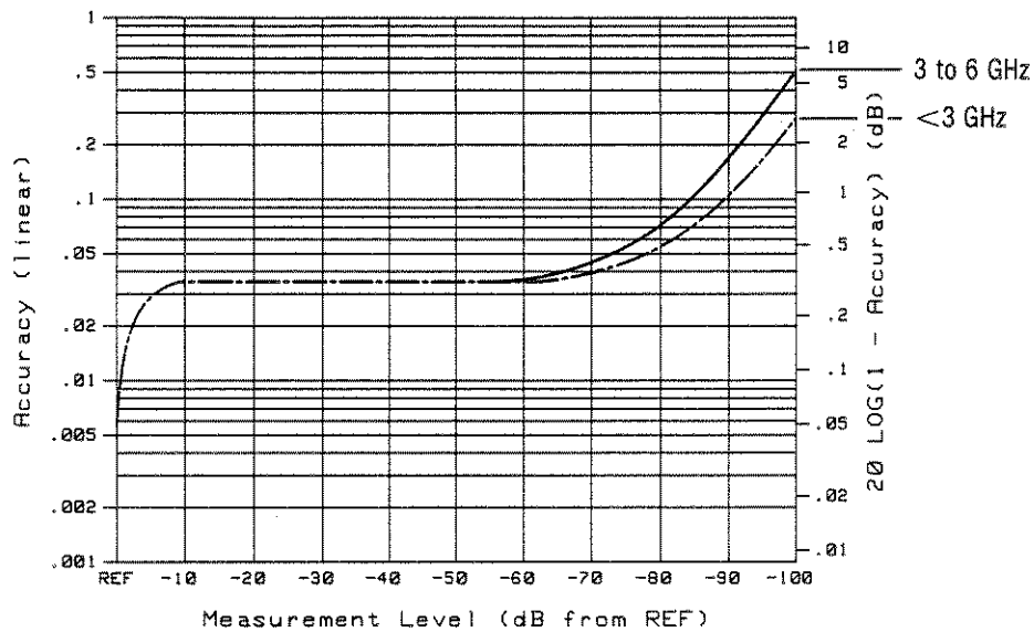
Figure 12. Worst-Case Magnitude Dynamic Accuracy Error
