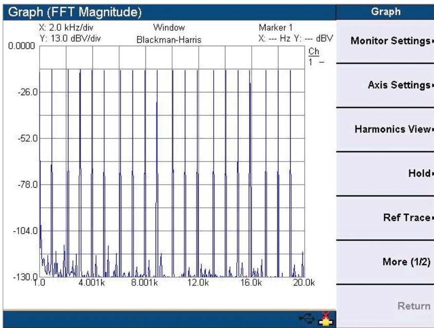
Figure 1. An example of a multitone signal consisting of 20 tones
