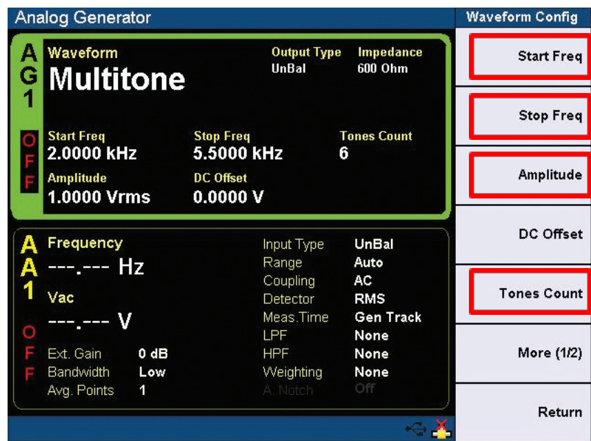
Figure 2. A standard multitone with 6 tones
