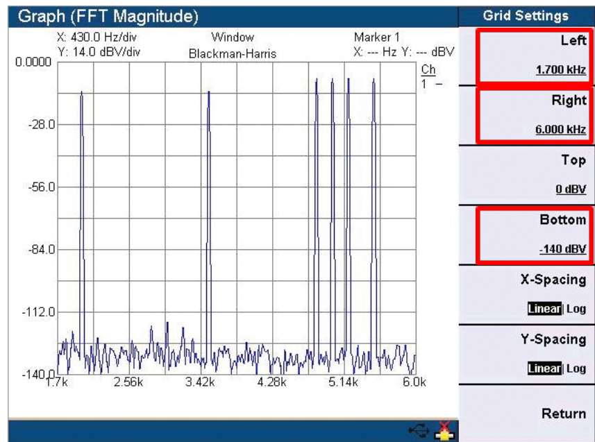
Figure 5. Spectrum of a custom multitone
